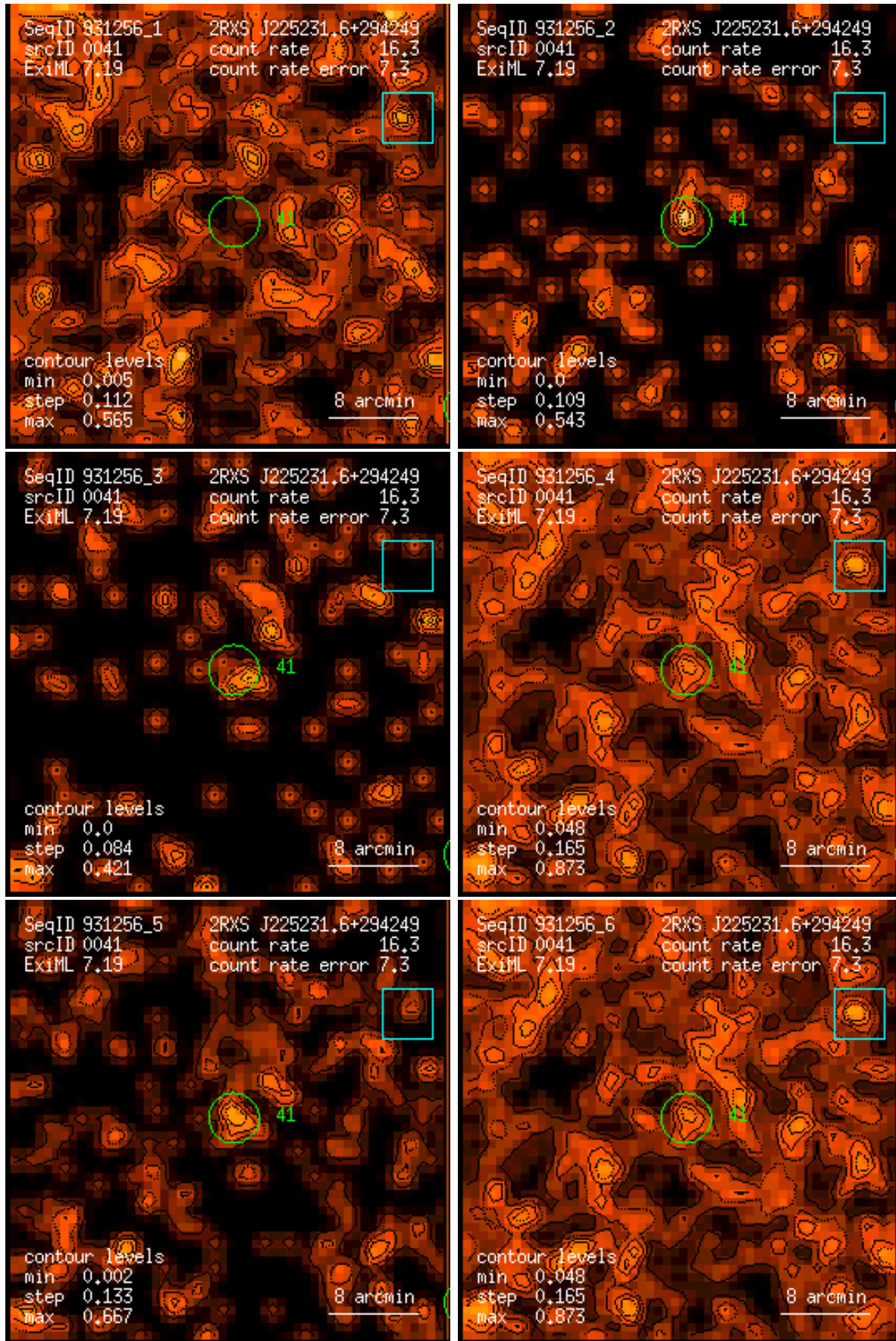
Figure 41: RASS 931256: detection 0041: band rate images, Gaussian filter: (1) PSPC channels 11 – 41, (2) 52 – 90, (3) 91 – 201, (4) 11 – 235, (5) 52 – 201, (6) 11 – 201. Broad band rates in counts/ks. Band rate contour levels in counts/ks/arcmin 2 .
