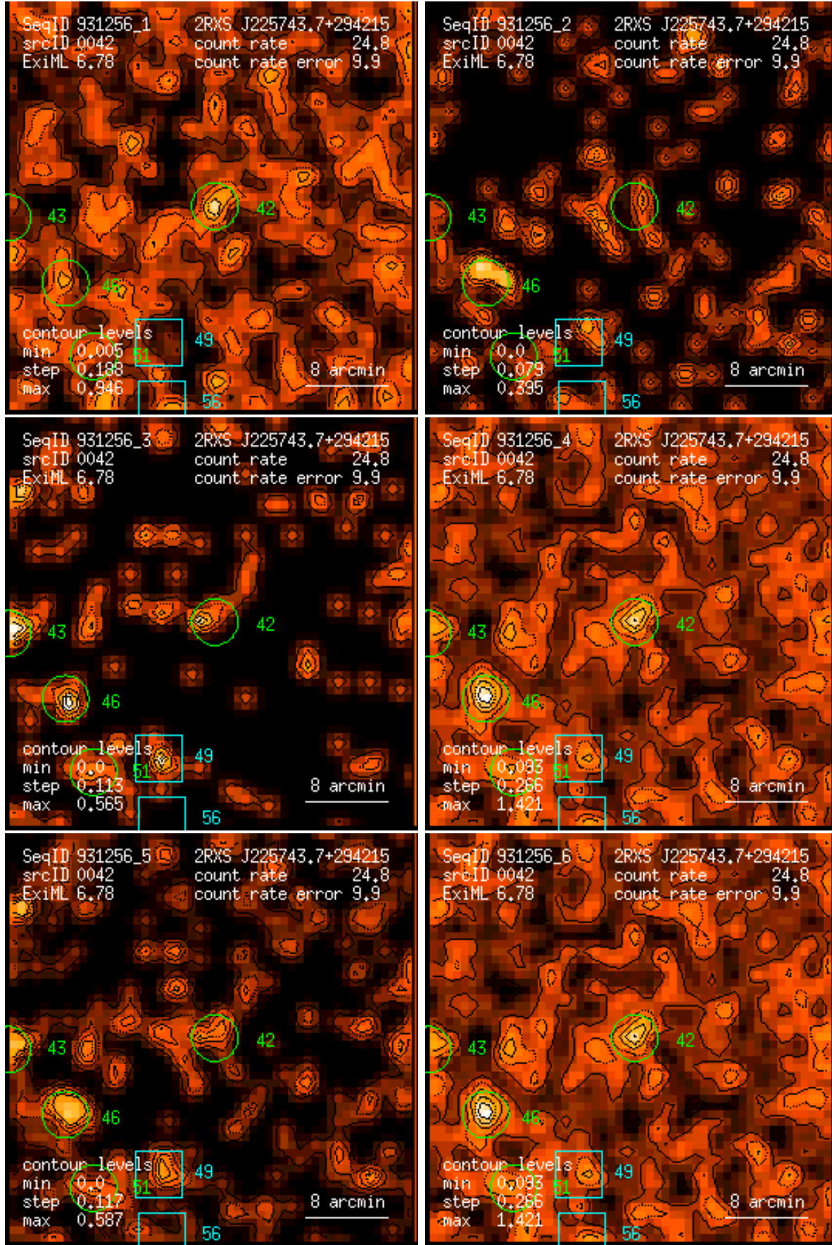
Figure 42: RASS 931256: detection 0042: band rate images, Gaussian filter: (1) PSPC channels 11 – 41, (2) 52 – 90, (3) 91 – 201, (4) 11 – 235, (5) 52 – 201, (6) 11 – 201. Broad band rates in counts/ks. Band rate contour levels in counts/ks/arcmin 2 .
