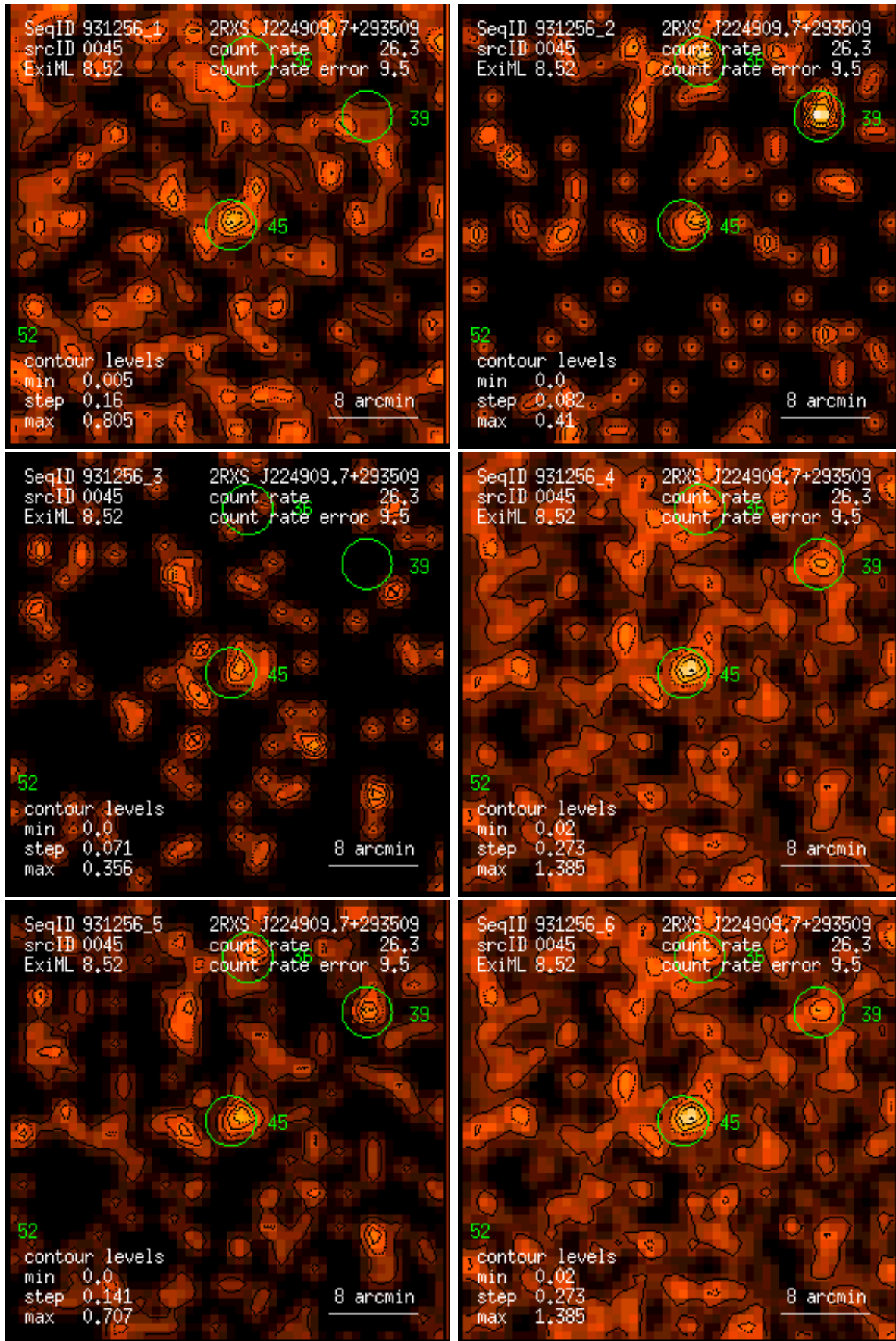
Figure 45: RASS 931256: detection 0045: band rate images, Gaussian filter: (1) PSPC channels 11 – 41, (2) 52 – 90, (3) 91 – 201, (4) 11 – 235, (5) 52 – 201, (6) 11 – 201. Broad band rates in counts/ks. Band rate contour levels in counts/ks/arcmin 2 .
