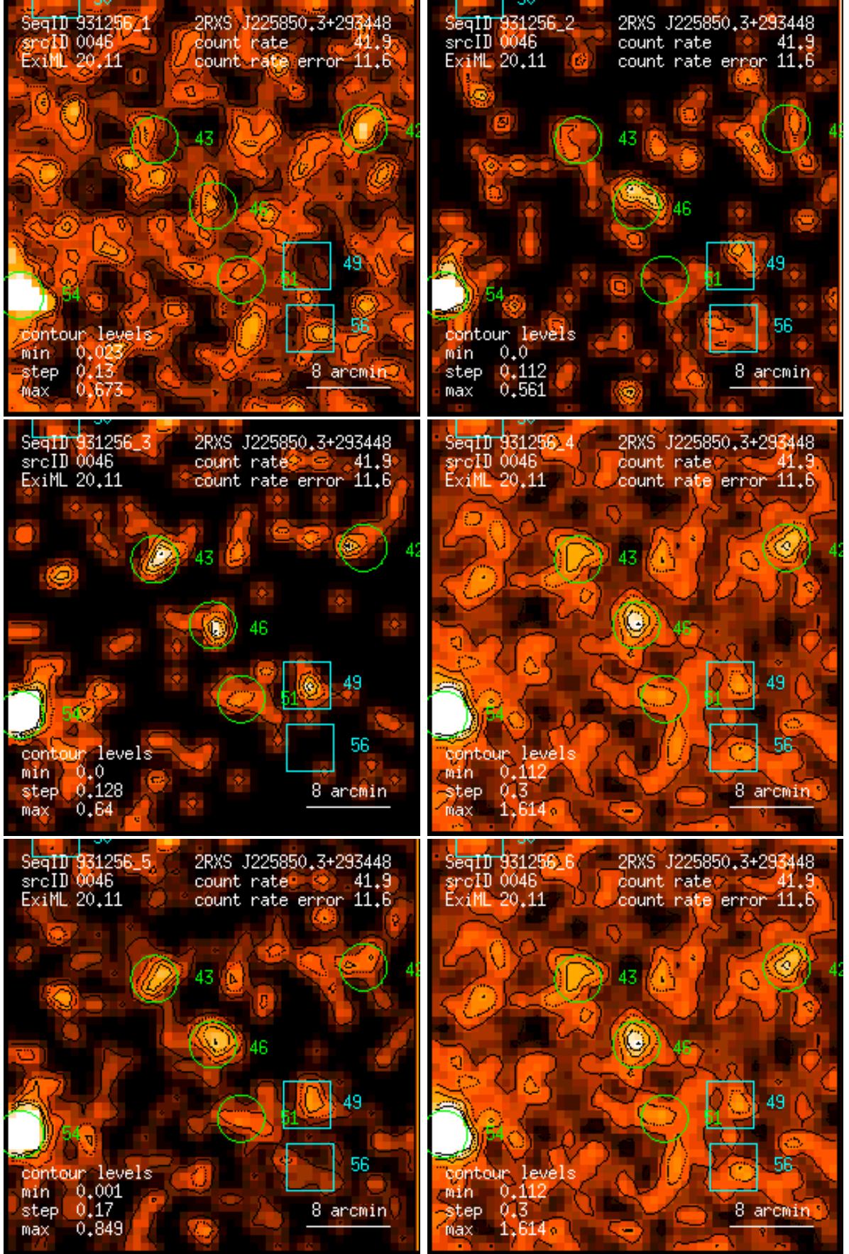
Figure 46: RASS 931256: detection 0046: band rate images, Gaussian filter: (1) PSPC channels 11 – 41, (2) 52 – 90, (3) 91 – 201, (4) 11 – 235, (5) 52 – 201, (6) 11 – 201. Broad band rates in counts/ks. Band rate contour levels in counts/ks/arcmin 2 .
