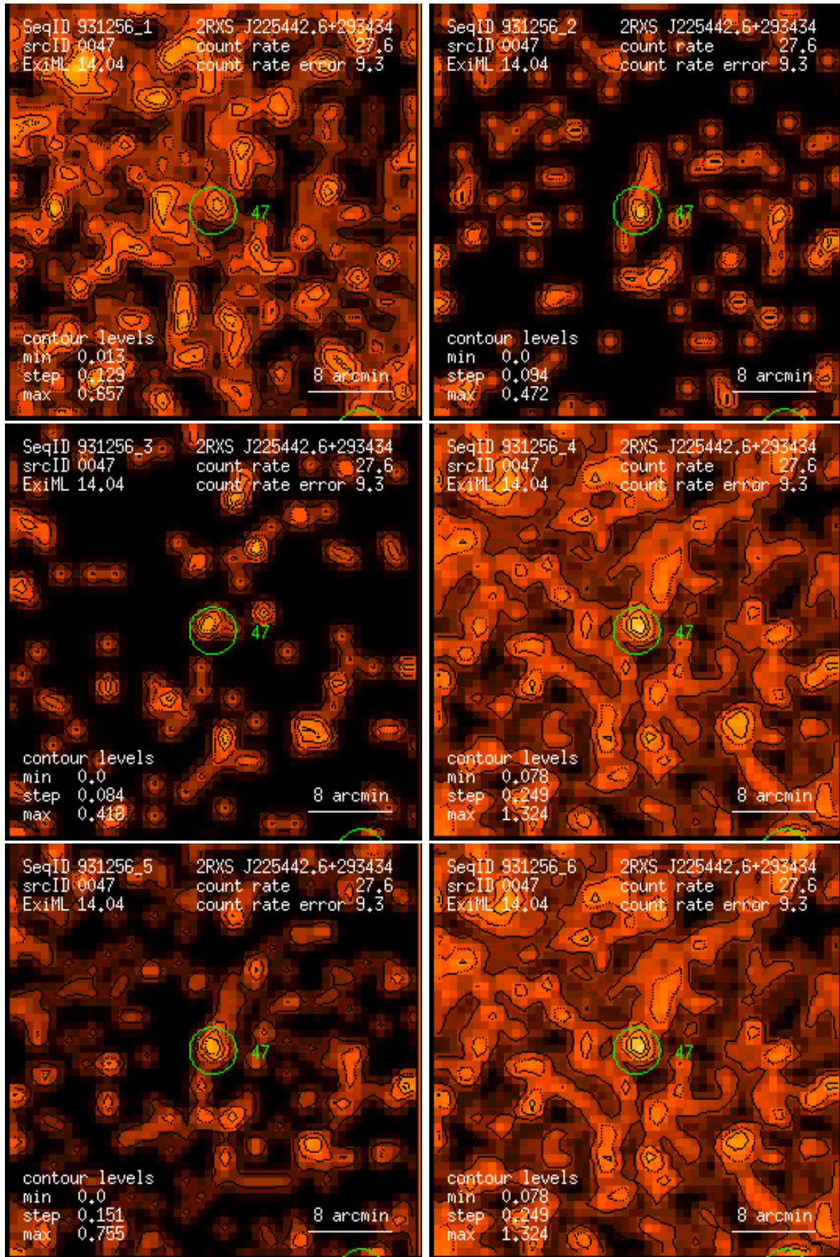
Figure 47: RASS 931256: detection 0047: band rate images, Gaussian filter: (1) PSPC channels 11 – 41, (2) 52 – 90, (3) 91 – 201, (4) 11 – 235, (5) 52 – 201, (6) 11 – 201. Broad band rates in counts/ks. Band rate contour levels in counts/ks/arcmin 2 .
