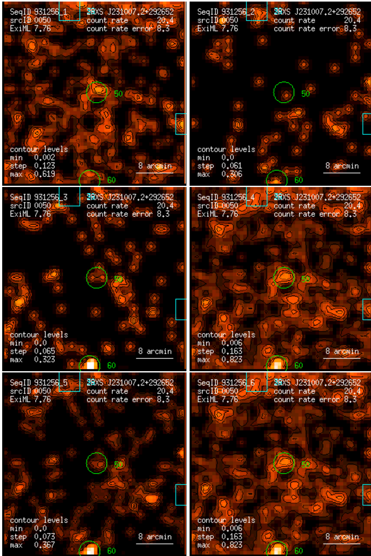
Figure 50: RASS 931256: detection 0050: band rate images, Gaussian filter: (1) PSPC channels 11 – 41, (2) 52 – 90, (3) 91 – 201, (4) 11 – 235, (5) 52 – 201, (6) 11 – 201. Broad band rates in counts/ks. Band rate contour levels in counts/ks/arcmin 2 .
