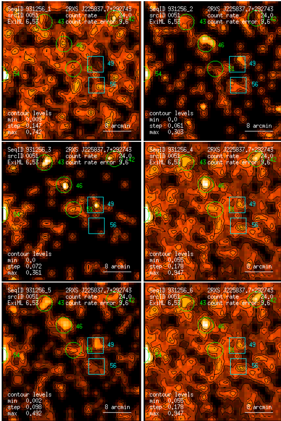
Figure 51: RASS 931256: detection 0051: band rate images, Gaussian filter: (1) PSPC channels 11 – 41, (2) 52 – 90, (3) 91 – 201, (4) 11 – 235, (5) 52 – 201, (6) 11 – 201. Broad band rates in counts/ks. Band rate contour levels in counts/ks/arcmin 2 .
