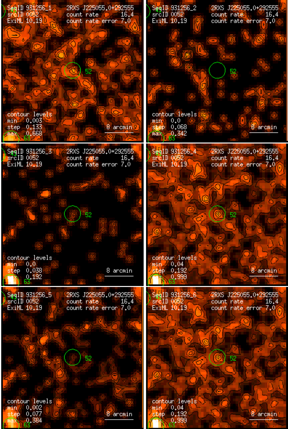
Figure 52: RASS 931256: detection 0052: band rate images, Gaussian filter: (1) PSPC channels 11 – 41, (2) 52 – 90, (3) 91 – 201, (4) 11 – 235, (5) 52 – 201, (6) 11 – 201. Broad band rates in counts/ks. Band rate contour levels in counts/ks/arcmin 2 .
