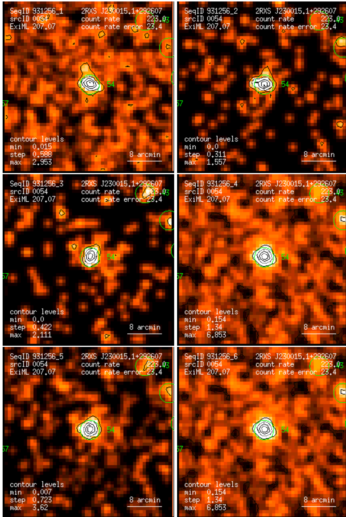
Figure 54: RASS 931256: detection 0054: band rate images, Gaussian filter: (1) PSPC channels 11 – 41, (2) 52 – 90, (3) 91 – 201, (4) 11 – 235, (5) 52 – 201, (6) 11 – 201. Broad band rates in counts/ks. Band rate contour levels in counts/ks/arcmin 2 .
