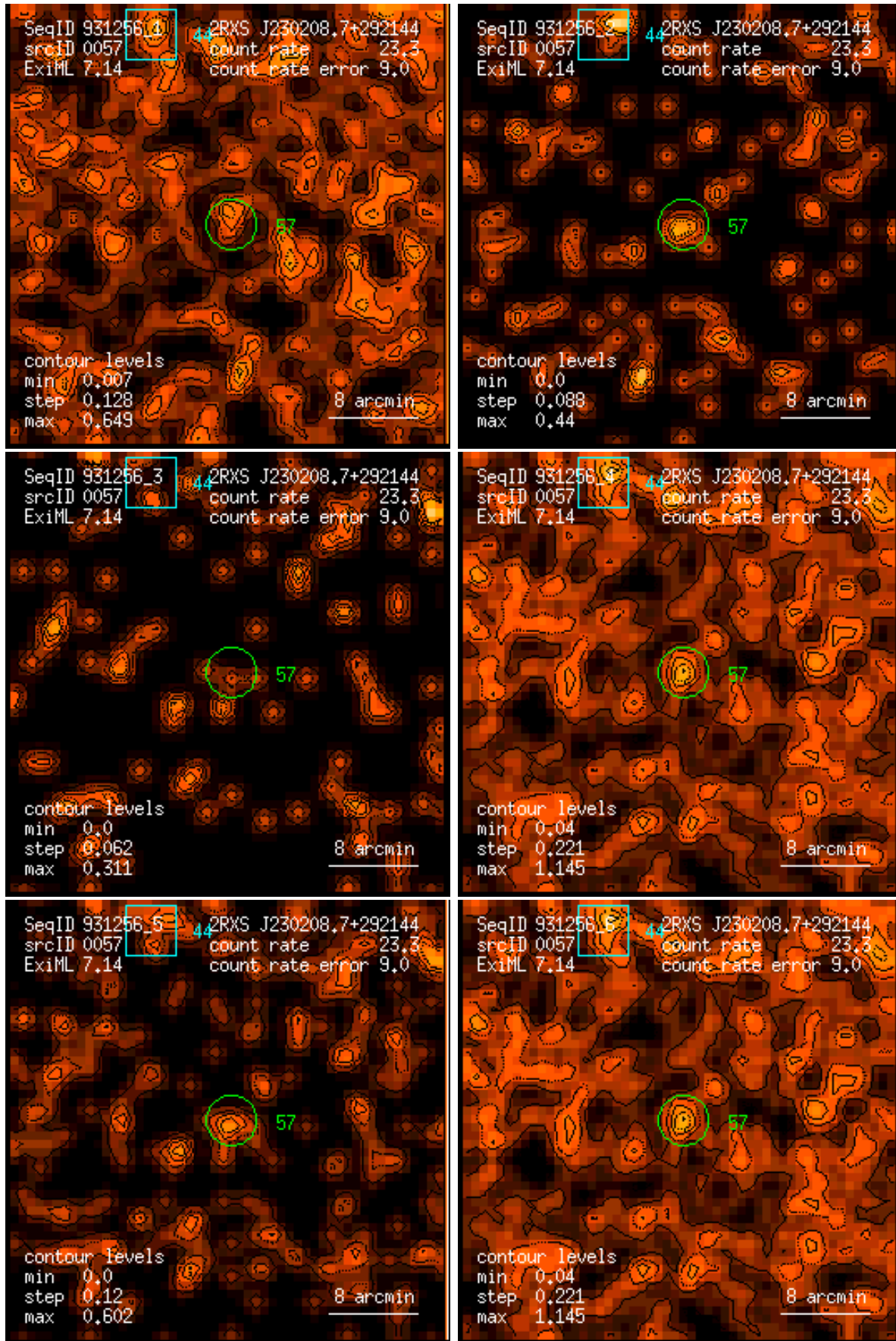
Figure 57: RASS 931256: detection 0057: band rate images, Gaussian filter: (1) PSPC channels 11 – 41, (2) 52 – 90, (3) 91 – 201, (4) 11 – 235, (5) 52 – 201, (6) 11 – 201. Broad band rates in counts/ks. Band rate contour levels in counts/ks/arcmin 2 .
