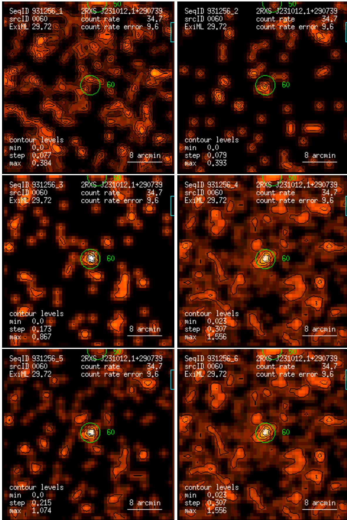
Figure 60: RASS 931256: detection 0060: band rate images, Gaussian filter: (1) PSPC channels 11 – 41, (2) 52 – 90, (3) 91 – 201, (4) 11 – 235, (5) 52 – 201, (6) 11 – 201. Broad band rates in counts/ks. Band rate contour levels in counts/ks/arcmin 2 .
