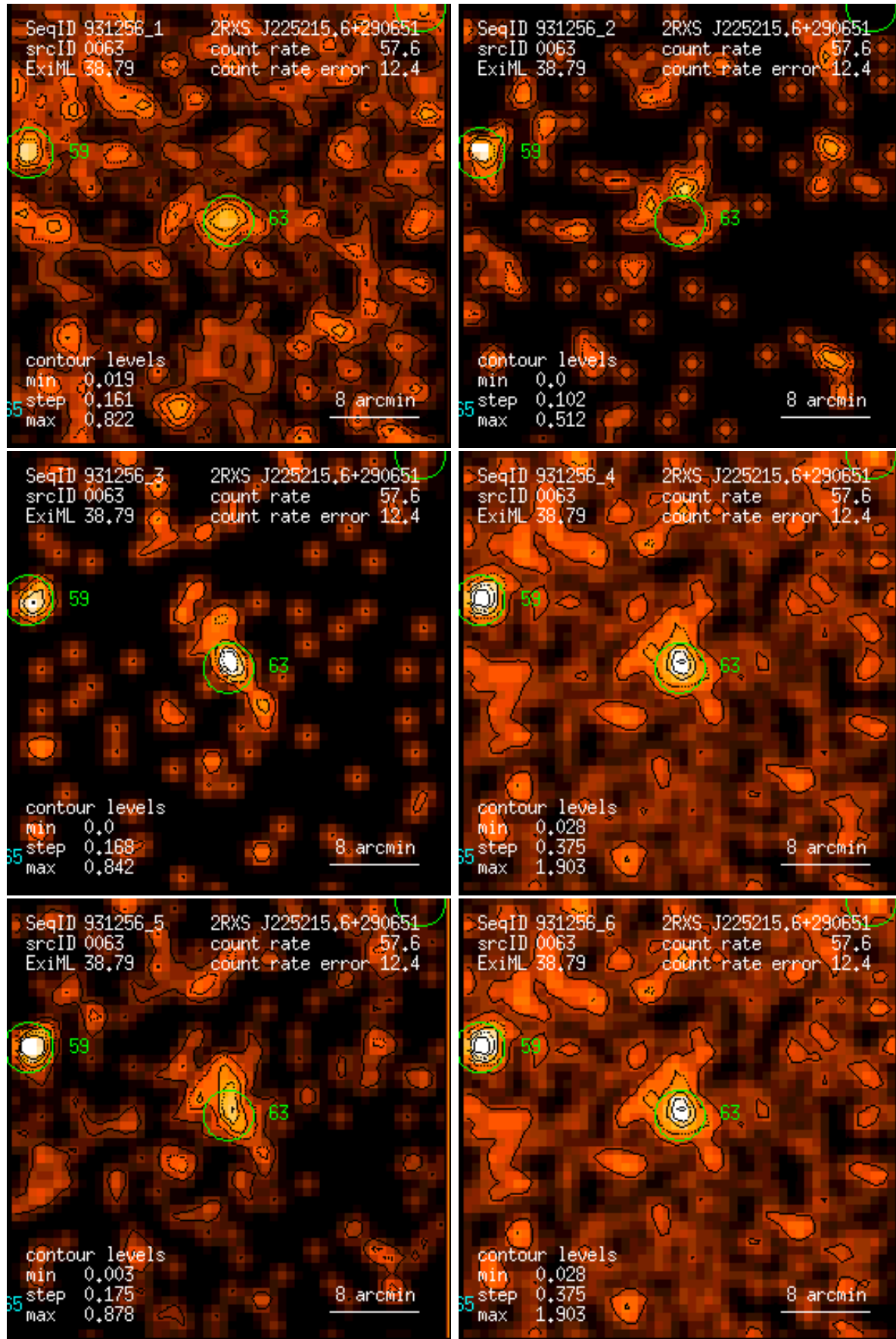
Figure 63: RASS 931256: detection 0063: band rate images, Gaussian filter: (1) PSPC channels 11 – 41, (2) 52 – 90, (3) 91 – 201, (4) 11 – 235, (5) 52 – 201, (6) 11 – 201. Broad band rates in counts/ks. Band rate contour levels in counts/ks/arcmin 2 .
