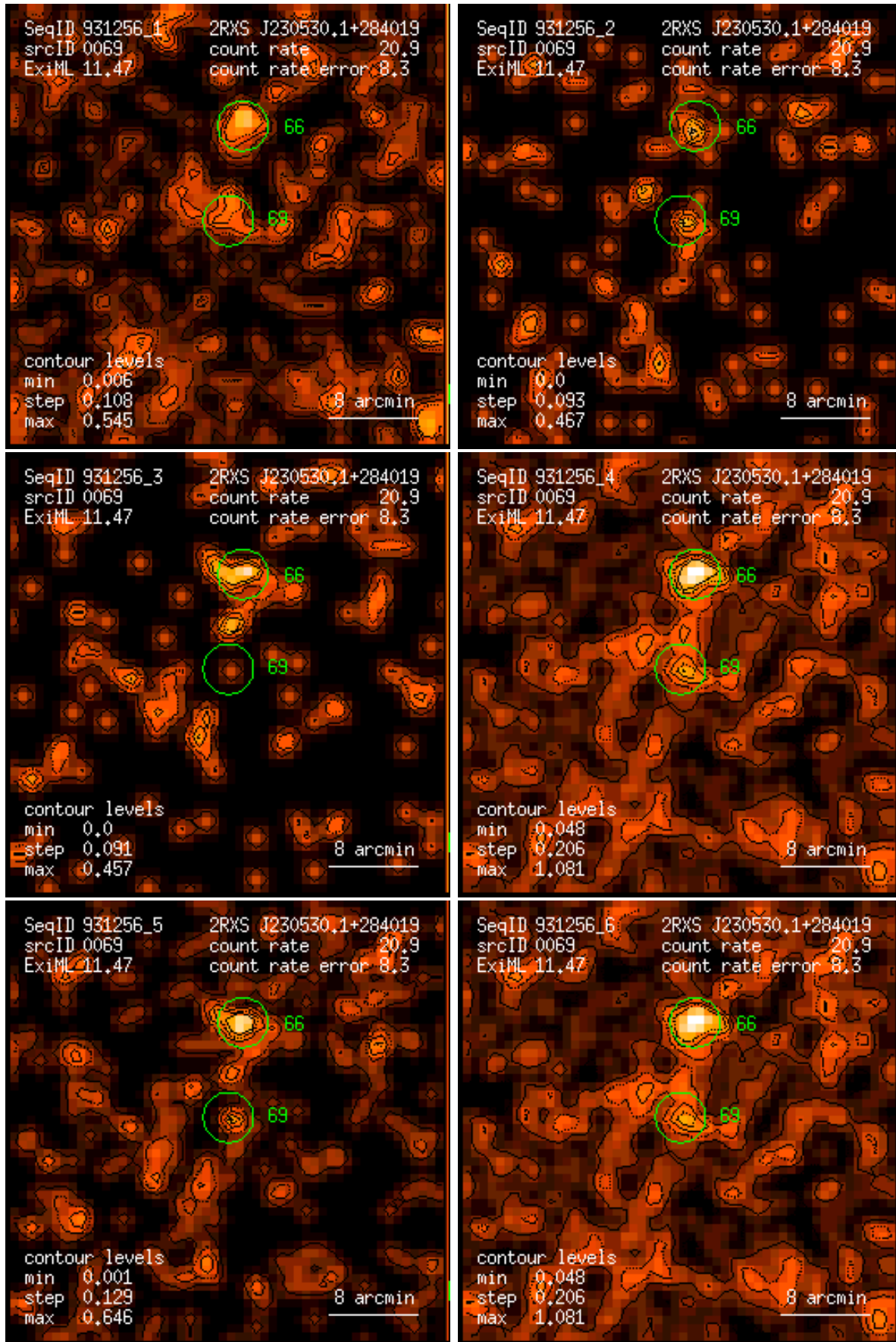
Figure 69: RASS 931256: detection 0069: band rate images, Gaussian filter: (1) PSPC channels 11 – 41, (2) 52 – 90, (3) 91 – 201, (4) 11 – 235, (5) 52 – 201, (6) 11 – 201. Broad band rates in counts/ks. Band rate contour levels in counts/ks/arcmin 2 .
