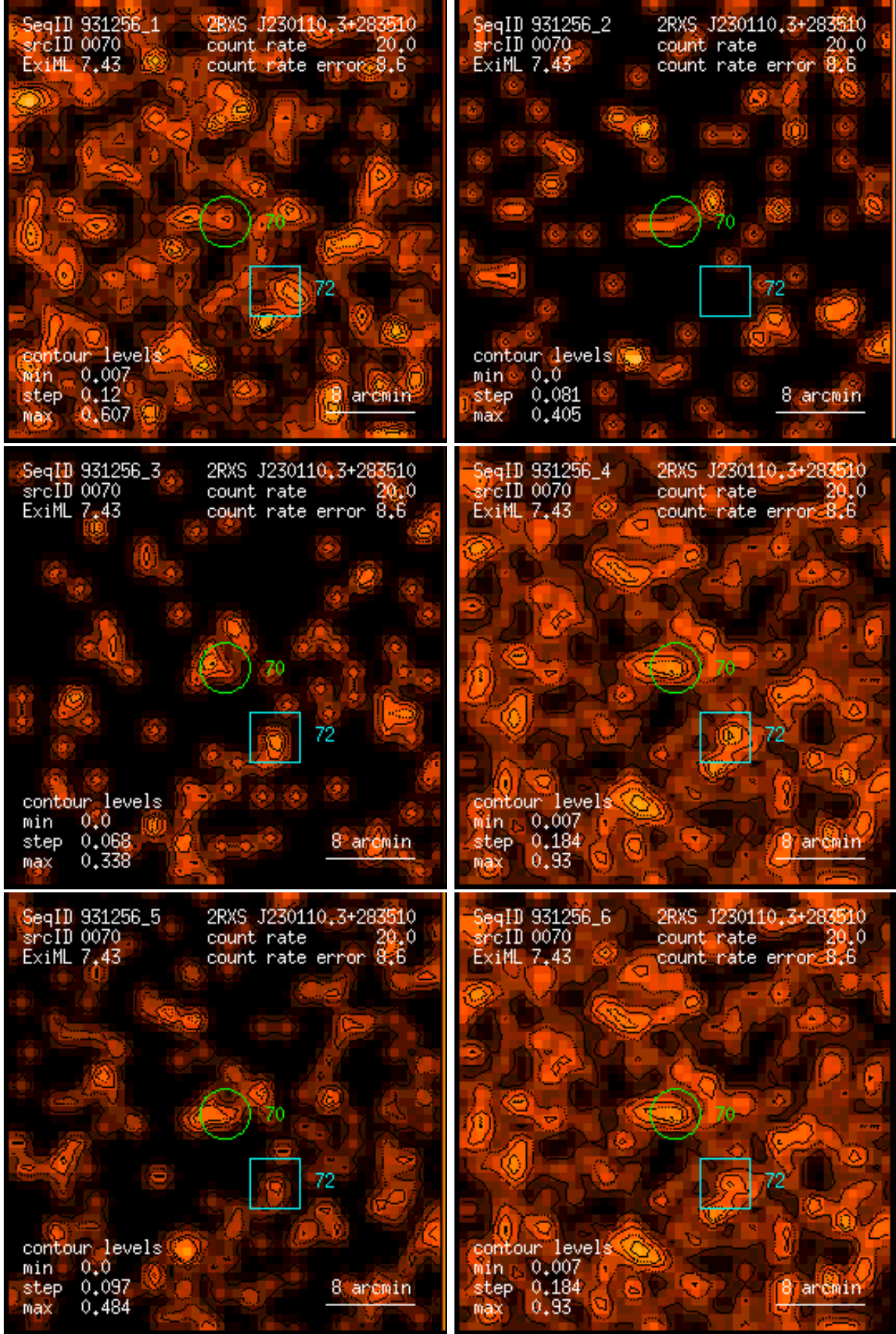
Figure 70: RASS 931256: detection 0070: band rate images, Gaussian filter: (1) PSPC channels 11 – 41, (2) 52 – 90, (3) 91 – 201, (4) 11 – 235, (5) 52 – 201, (6) 11 – 201. Broad band rates in counts/ks. Band rate contour levels in counts/ks/arcmin 2 .
