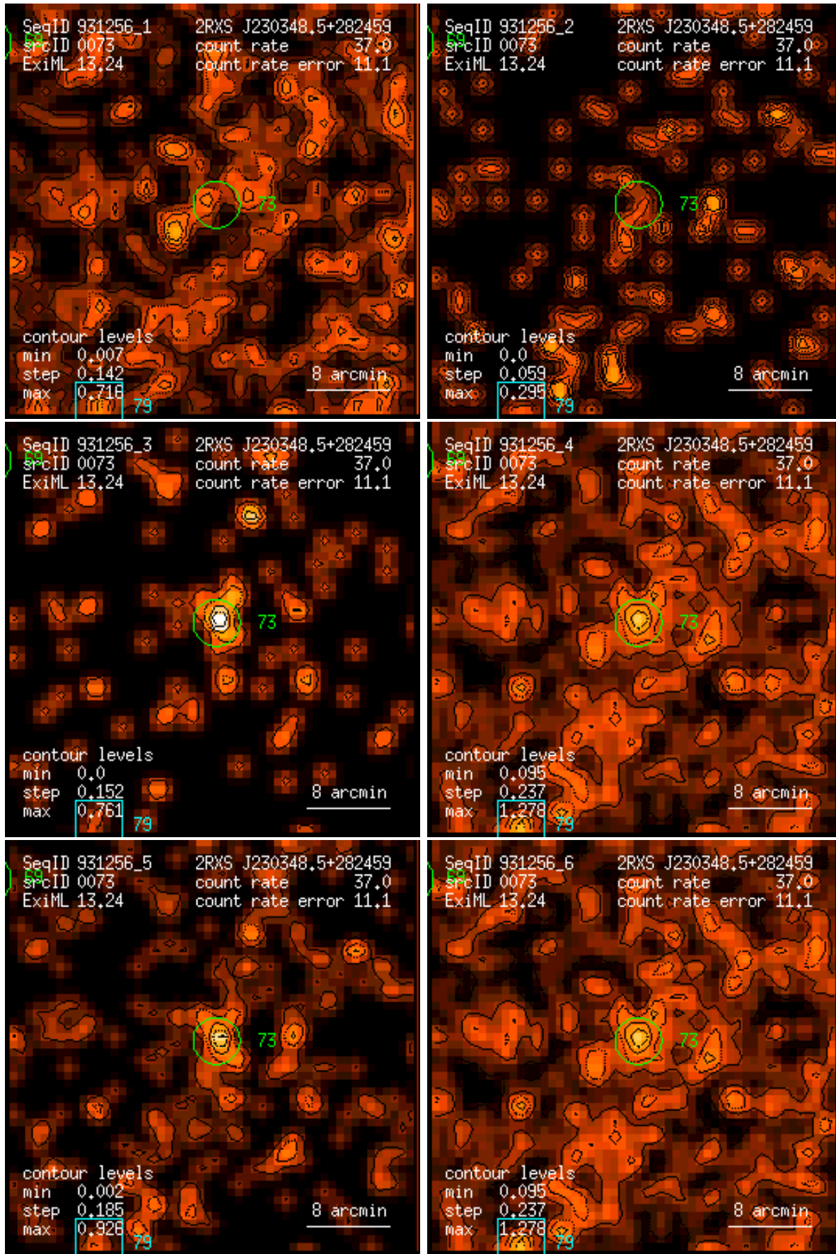
Figure 73: RASS 931256: detection 0073: band rate images, Gaussian filter: (1) PSPC channels 11 – 41, (2) 52 – 90, (3) 91 – 201, (4) 11 – 235, (5) 52 – 201, (6) 11 – 201. Broad band rates in counts/ks. Band rate contour levels in counts/ks/arcmin 2 .
