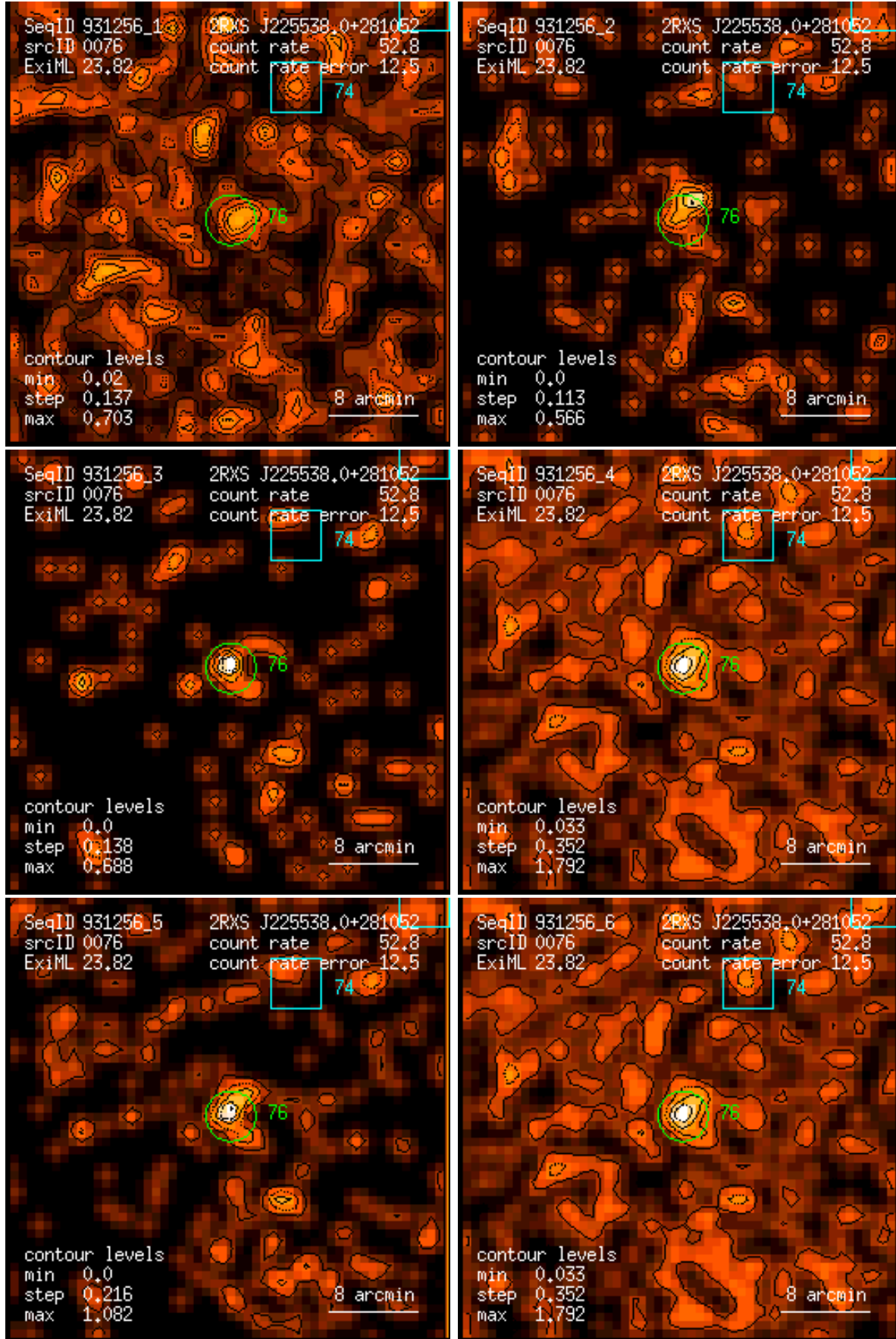
Figure 76: RASS 931256: detection 0076: band rate images, Gaussian filter: (1) PSPC channels 11 – 41, (2) 52 – 90, (3) 91 – 201, (4) 11 – 235, (5) 52 – 201, (6) 11 – 201. Broad band rates in counts/ks. Band rate contour levels in counts/ks/arcmin 2 .
