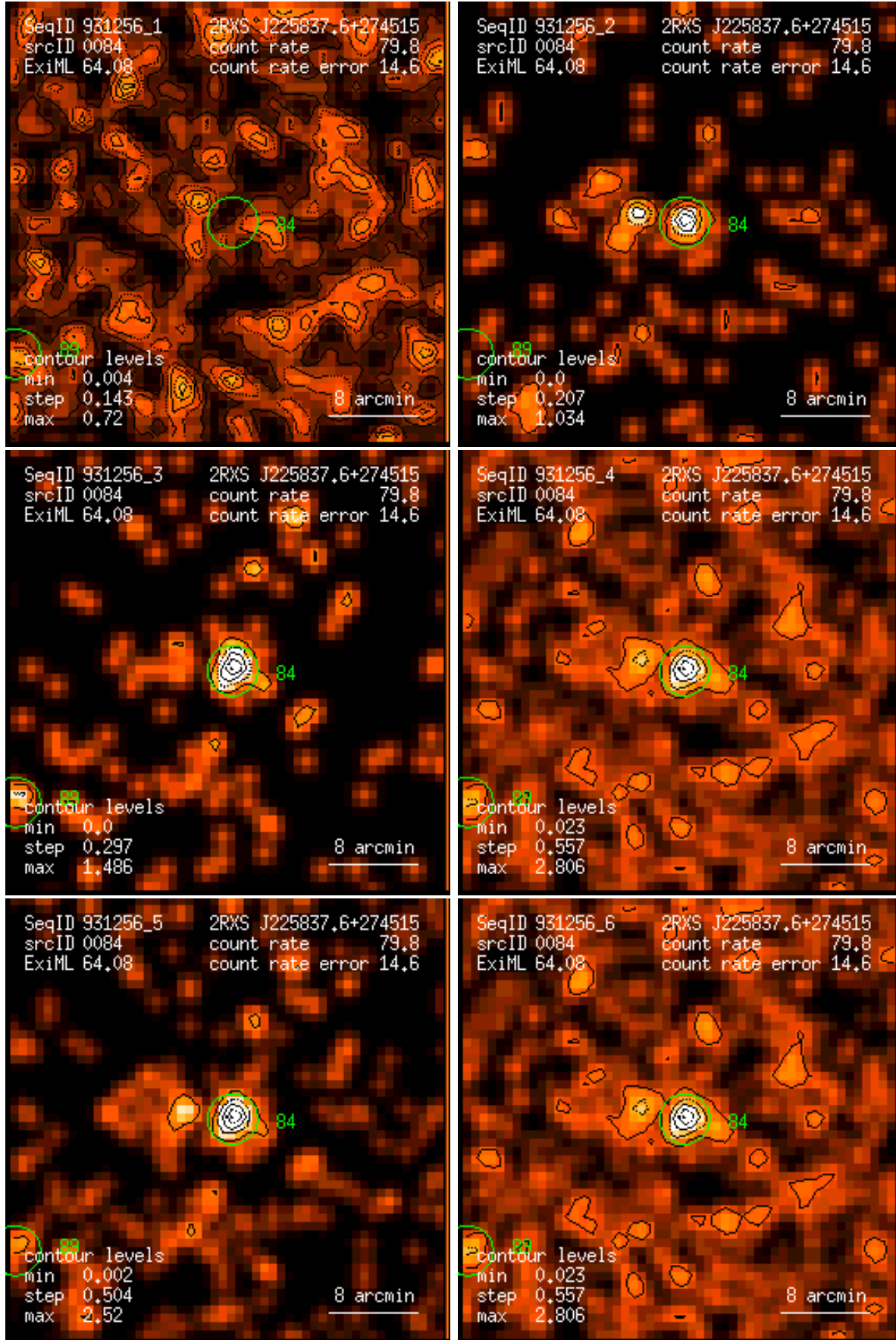
Figure 84: RASS 931256: detection 0084: band rate images, Gaussian filter: (1) PSPC channels 11 – 41, (2) 52 – 90, (3) 91 – 201, (4) 11 – 235, (5) 52 – 201, (6) 11 – 201. Broad band rates in counts/ks. Band rate contour levels in counts/ks/arcmin 2 .
