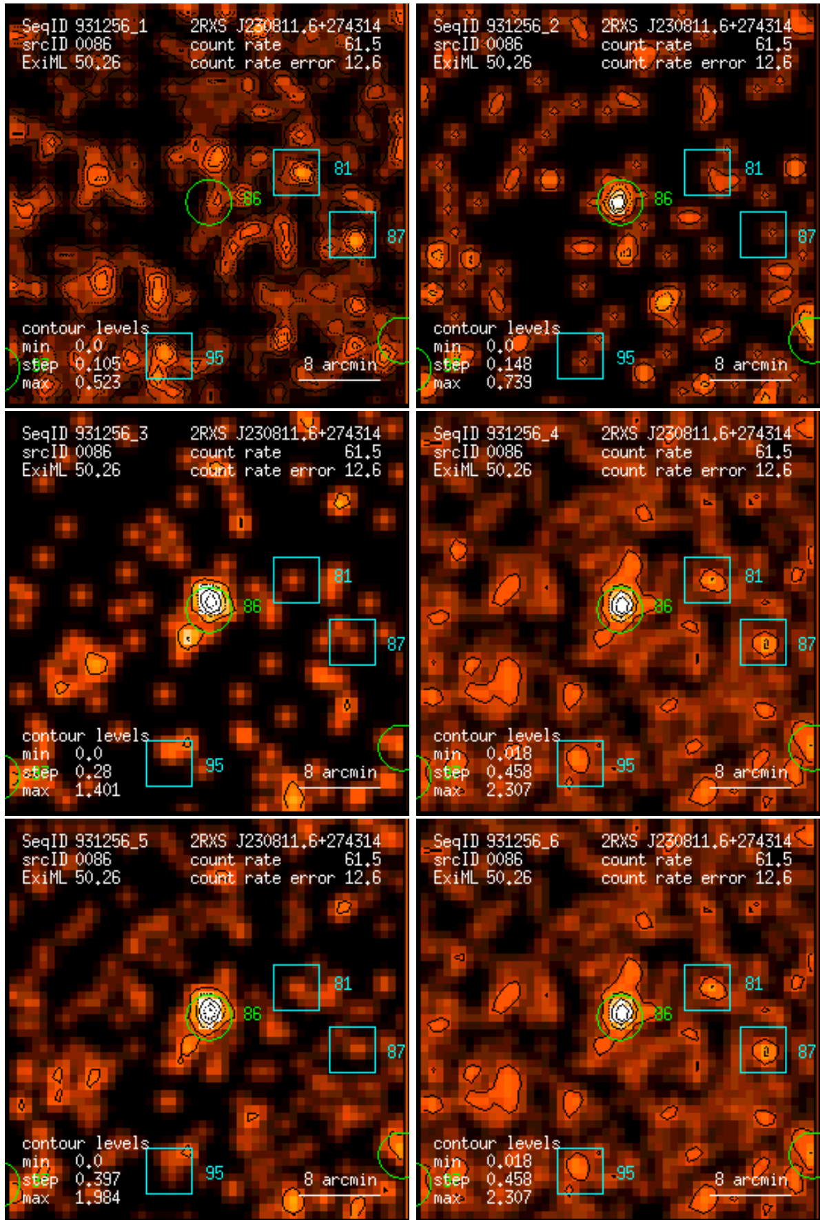
Figure 86: RASS 931256: detection 0086: band rate images, Gaussian filter: (1) PSPC channels 11 – 41, (2) 52 – 90, (3) 91 – 201, (4) 11 – 235, (5) 52 – 201, (6) 11 – 201. Broad band rates in counts/ks. Band rate contour levels in counts/ks/arcmin 2 .
