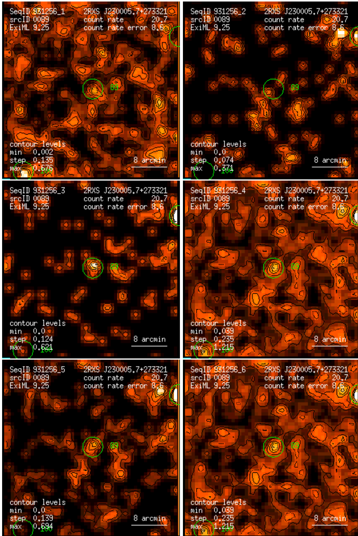
Figure 89: RASS 931256: detection 0089: band rate images, Gaussian filter: (1) PSPC channels 11 – 41, (2) 52 – 90, (3) 91 – 201, (4) 11 – 235, (5) 52 – 201, (6) 11 – 201. Broad band rates in counts/ks. Band rate contour levels in counts/ks/arcmin 2 .
