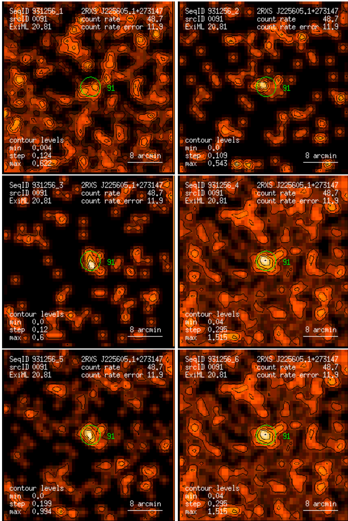
Figure 91: RASS 931256: detection 0091: band rate images, Gaussian filter: (1) PSPC channels 11 – 41, (2) 52 – 90, (3) 91 – 201, (4) 11 – 235, (5) 52 – 201, (6) 11 – 201. Broad band rates in counts/ks. Band rate contour levels in counts/ks/arcmin 2 .
