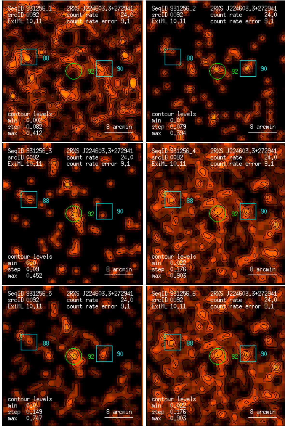
Figure 92: RASS 931256: detection 0092: band rate images, Gaussian filter: (1) PSPC channels 11 – 41, (2) 52 – 90, (3) 91 – 201, (4) 11 – 235, (5) 52 – 201, (6) 11 – 201. Broad band rates in counts/ks. Band rate contour levels in counts/ks/arcmin 2 .
