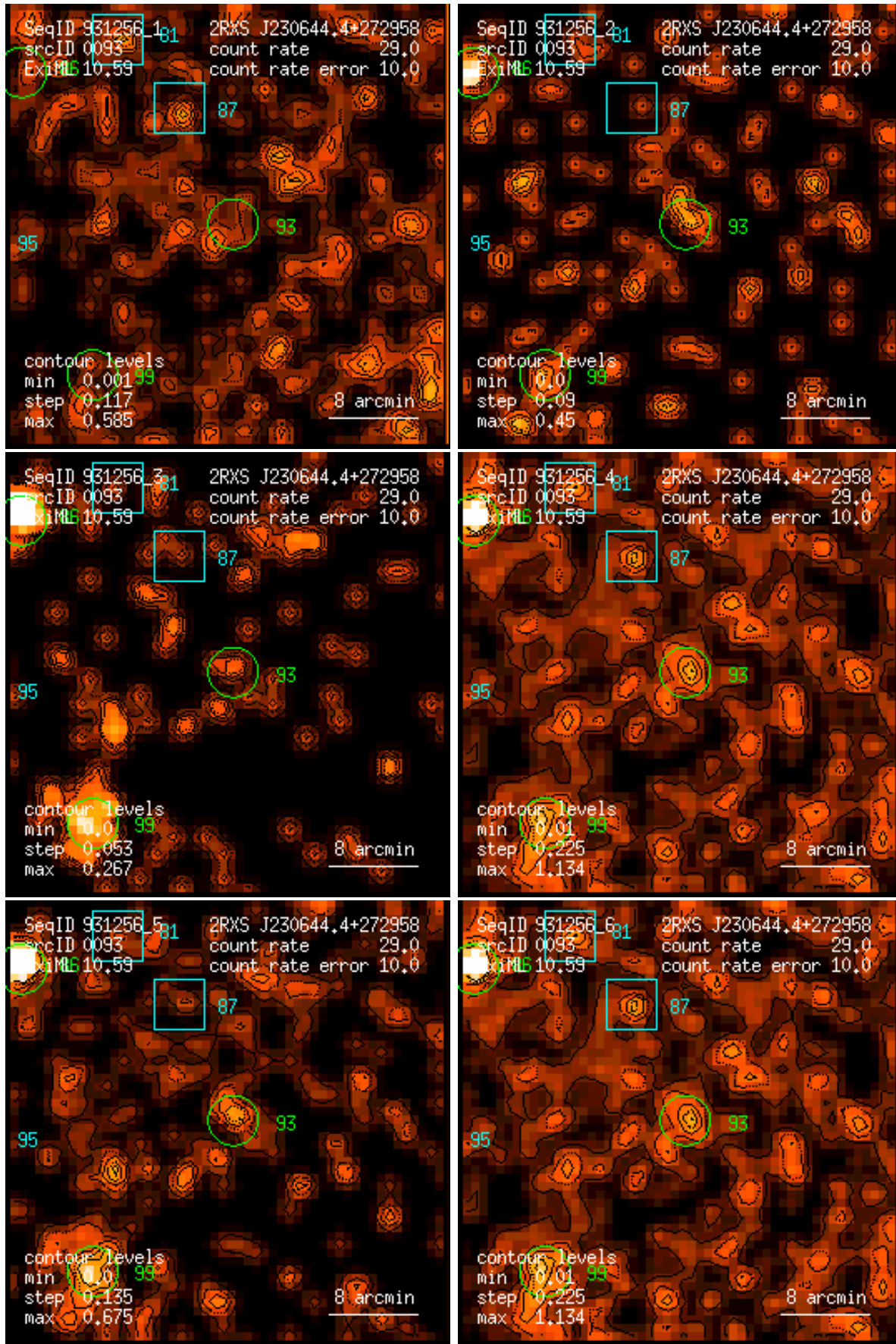
Figure 93: RASS 931256: detection 0093: band rate images, Gaussian filter: (1) PSPC channels 11 – 41, (2) 52 – 90, (3) 91 – 201, (4) 11 – 235, (5) 52 – 201, (6) 11 – 201. Broad band rates in counts/ks. Band rate contour levels in counts/ks/arcmin 2 .
