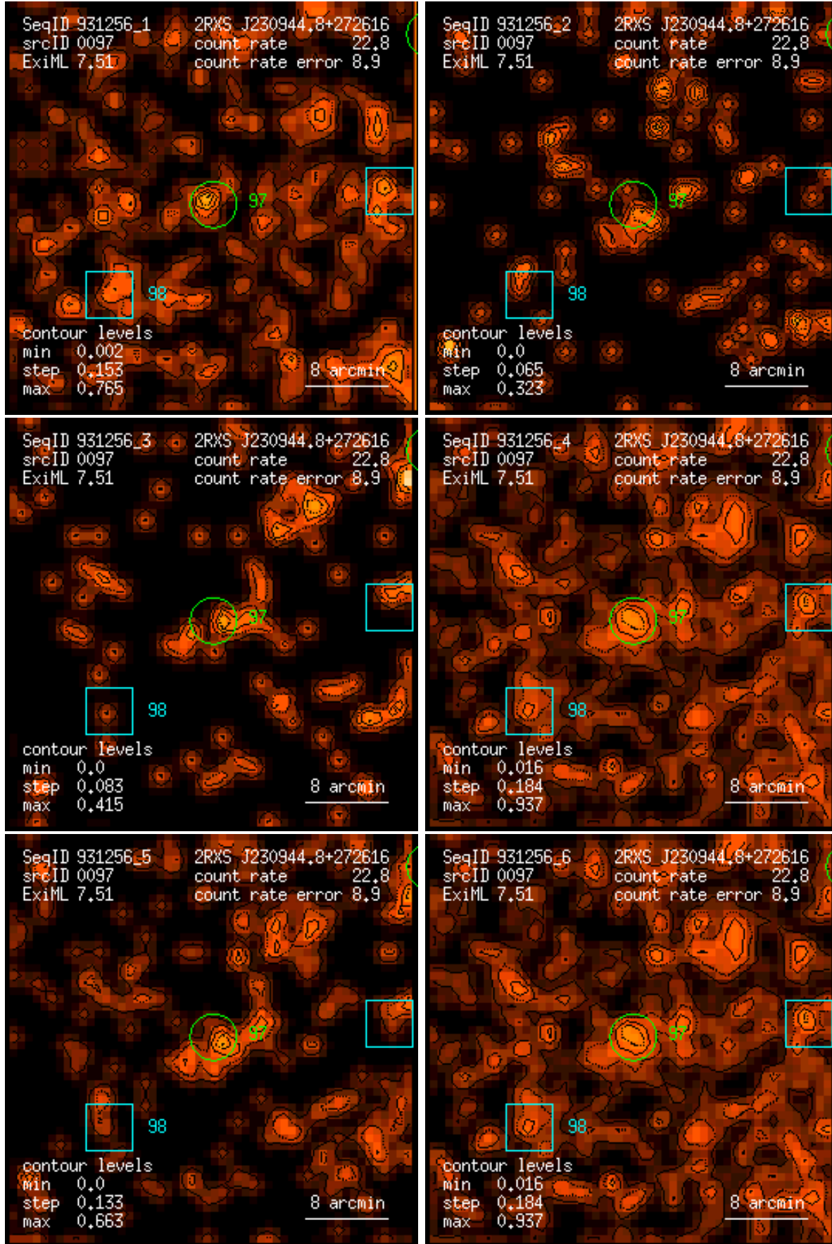
Figure 97: RASS 931256: detection 0097: band rate images, Gaussian filter: (1) PSPC channels 11 – 41, (2) 52 – 90, (3) 91 – 201, (4) 11 – 235, (5) 52 – 201, (6) 11 – 201. Broad band rates in counts/ks. Band rate contour levels in counts/ks/arcmin 2 .
