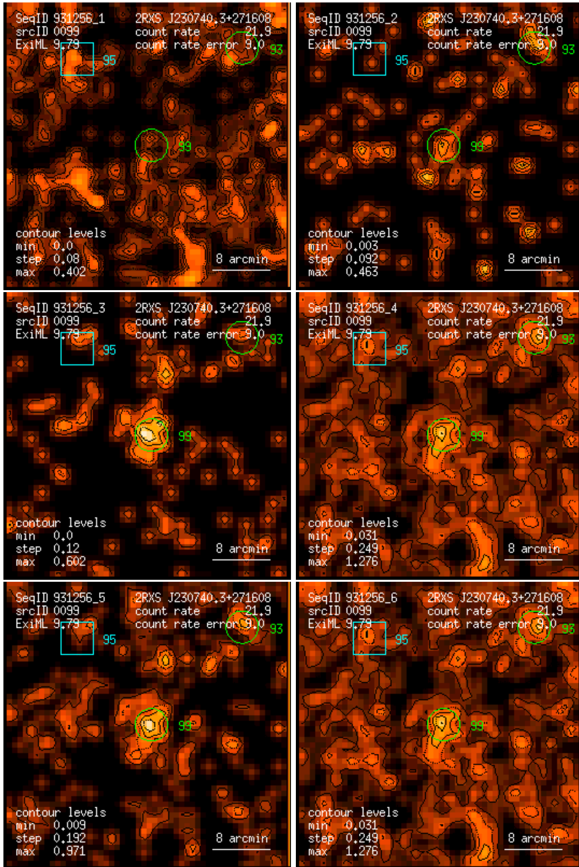
Figure 99: RASS 931256: detection 0099: band rate images, Gaussian filter: (1) PSPC channels 11 – 41, (2) 52 – 90, (3) 91 – 201, (4) 11 – 235, (5) 52 – 201, (6) 11 – 201. Broad band rates in counts/ks. Band rate contour levels in counts/ks/arcmin 2 .
