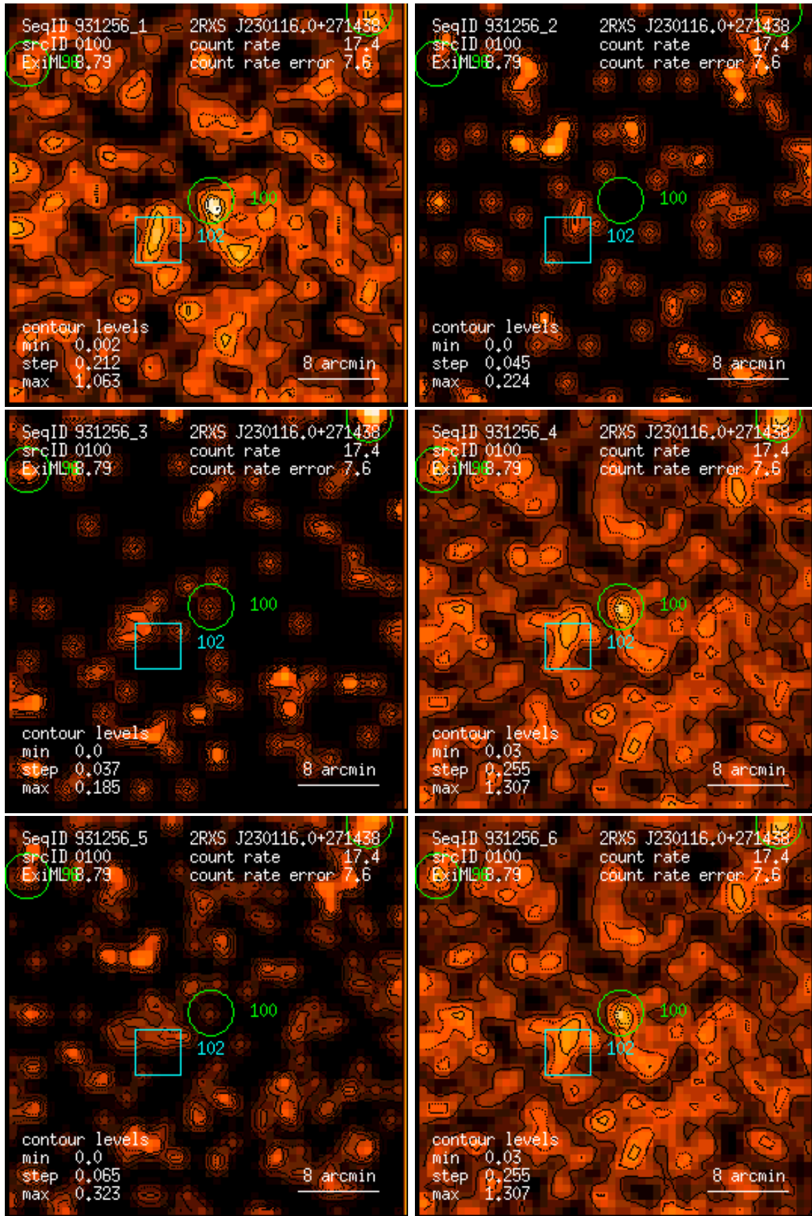
Figure 100: RASS 931256: detection 0100: band rate images, Gaussian filter: (1) PSPC channels 11 – 41, (2) 52 – 90, (3) 91 – 201, (4) 11 – 235, (5) 52 – 201, (6) 11 – 201. Broad band rates in counts/ks. Band rate contour levels in counts/ks/arcmin 2 .
