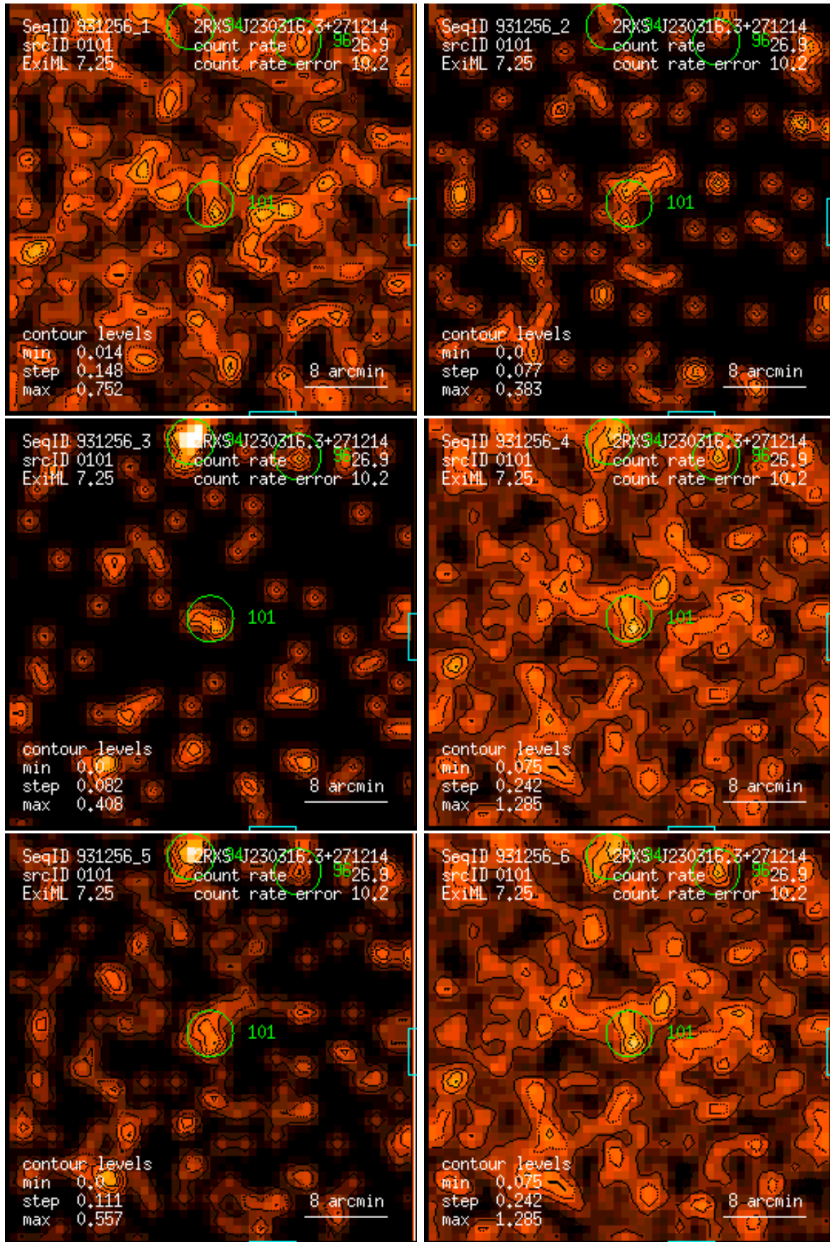
Figure 101: RASS 931256: detection 0101: band rate images, Gaussian filter: (1) PSPC channels 11 – 41, (2) 52 – 90, (3) 91 – 201, (4) 11 – 235, (5) 52 – 201, (6) 11 – 201. Broad band rates in counts/ks. Band rate contour levels in counts/ks/arcmin 2 .
