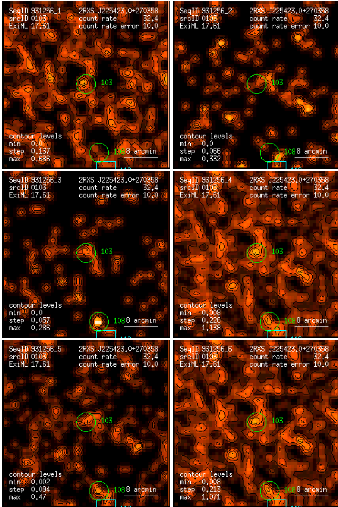
Figure 103: RASS 931256: detection 0103: band rate images, Gaussian filter: (1) PSPC channels 11 – 41, (2) 52 – 90, (3) 91 – 201, (4) 11 – 235, (5) 52 – 201, (6) 11 – 201. Broad band rates in counts/ks. Band rate contour levels in counts/ks/arcmin 2 .
