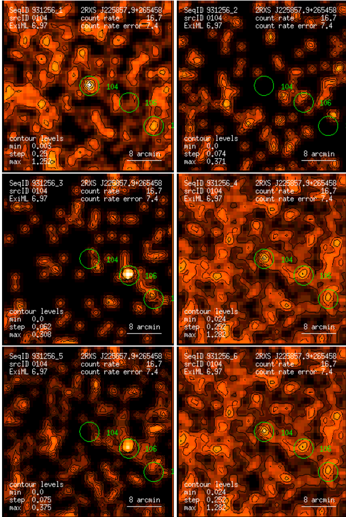
Figure 104: RASS 931256: detection 0104: band rate images, Gaussian filter: (1) PSPC channels 11 – 41, (2) 52 – 90, (3) 91 – 201, (4) 11 – 235, (5) 52 – 201, (6) 11 – 201. Broad band rates in counts/ks. Band rate contour levels in counts/ks/arcmin 2 .
