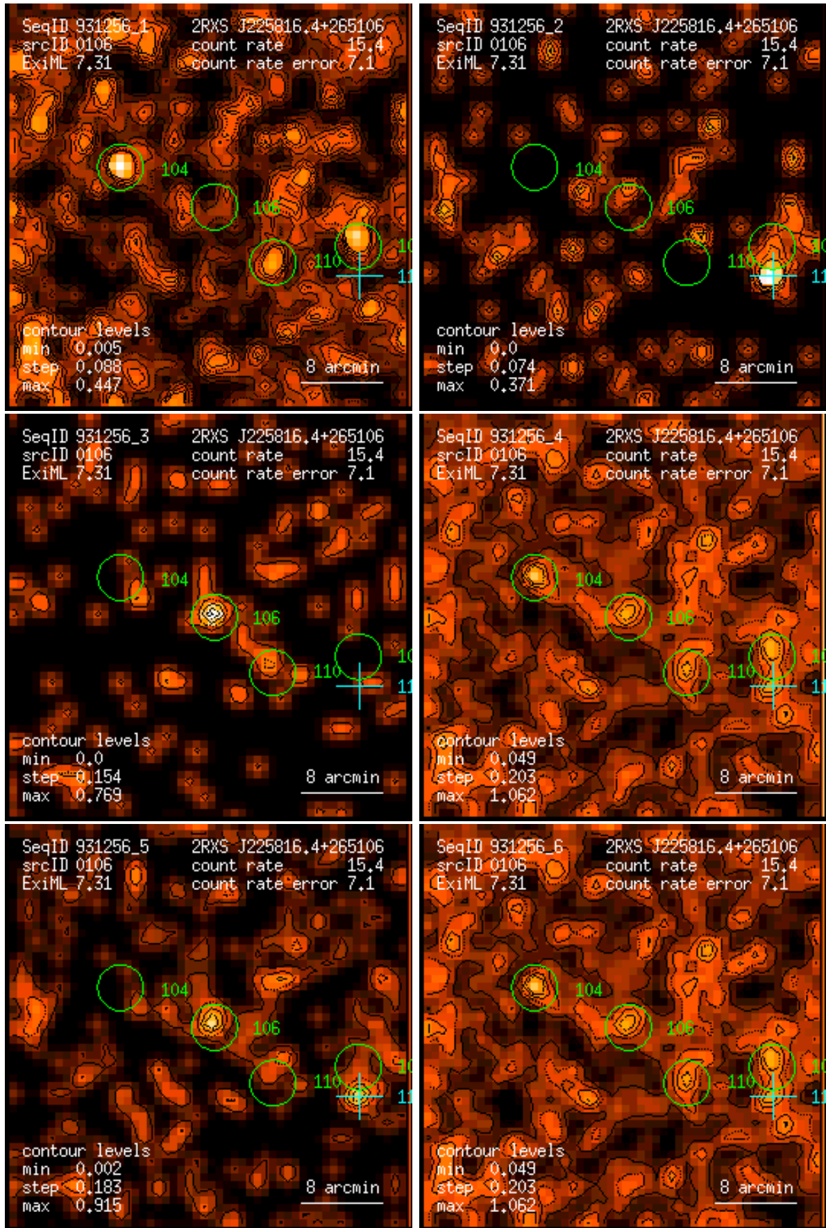
Figure 106: RASS 931256: detection 0106: band rate images, Gaussian filter: (1) PSPC channels 11 – 41, (2) 52 – 90, (3) 91 – 201, (4) 11 – 235, (5) 52 – 201, (6) 11 – 201. Broad band rates in counts/ks. Band rate contour levels in counts/ks/arcmin 2 .
