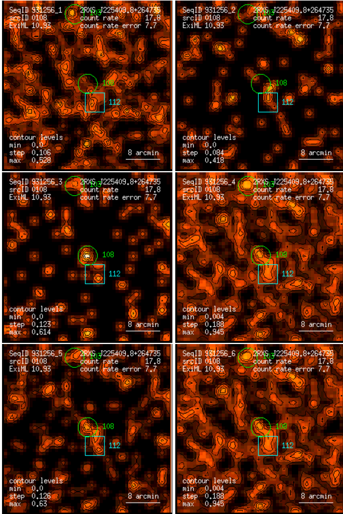
Figure 108: RASS 931256: detection 0108: band rate images, Gaussian filter: (1) PSPC channels 11 – 41, (2) 52 – 90, (3) 91 – 201, (4) 11 – 235, (5) 52 – 201, (6) 11 – 201. Broad band rates in counts/ks. Band rate contour levels in counts/ks/arcmin 2 .
