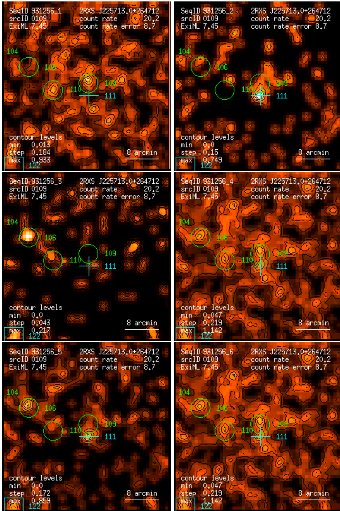
Figure 109: RASS 931256: detection 0109: band rate images, Gaussian filter: (1) PSPC channels 11 – 41, (2) 52 – 90, (3) 91 – 201, (4) 11 – 235, (5) 52 – 201, (6) 11 – 201. Broad band rates in counts/ks. Band rate contour levels in counts/ks/arcmin 2 .
