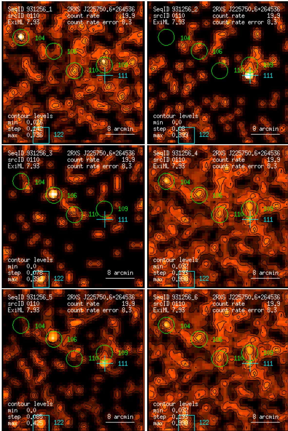
Figure 110: RASS 931256: detection 0110: band rate images, Gaussian filter: (1) PSPC channels 11 – 41, (2) 52 – 90, (3) 91 – 201, (4) 11 – 235, (5) 52 – 201, (6) 11 – 201. Broad band rates in counts/ks. Band rate contour levels in counts/ks/arcmin 2 .
