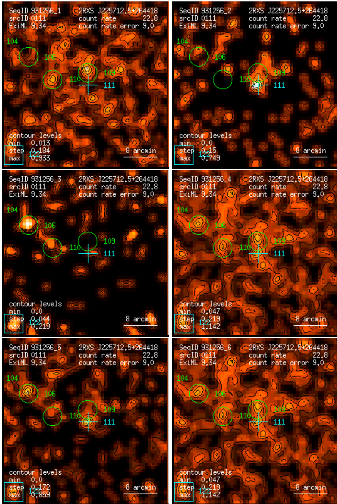
Figure 111: RASS 931256: detection 0111: band rate images, Gaussian filter: (1) PSPC channels 11 – 41, (2) 52 – 90, (3) 91 – 201, (4) 11 – 235, (5) 52 – 201, (6) 11 – 201. Broad band rates in counts/ks. Band rate contour levels in counts/ks/arcmin 2 .
