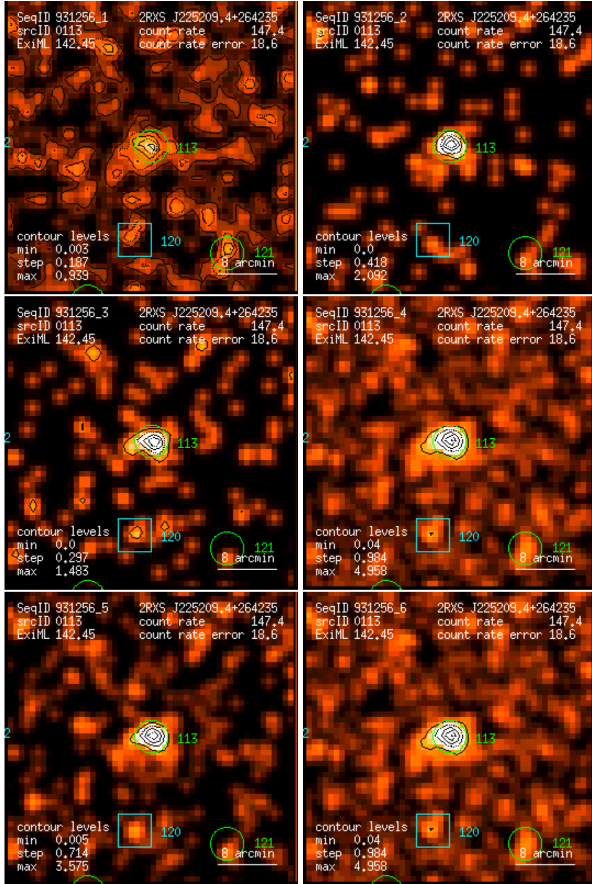
Figure 113: RASS 931256: detection 0113: band rate images, Gaussian filter: (1) PSPC channels 11 – 41, (2) 52 – 90, (3) 91 – 201, (4) 11 – 235, (5) 52 – 201, (6) 11 – 201. Broad band rates in counts/ks. Band rate contour levels in counts/ks/arcmin 2 .
