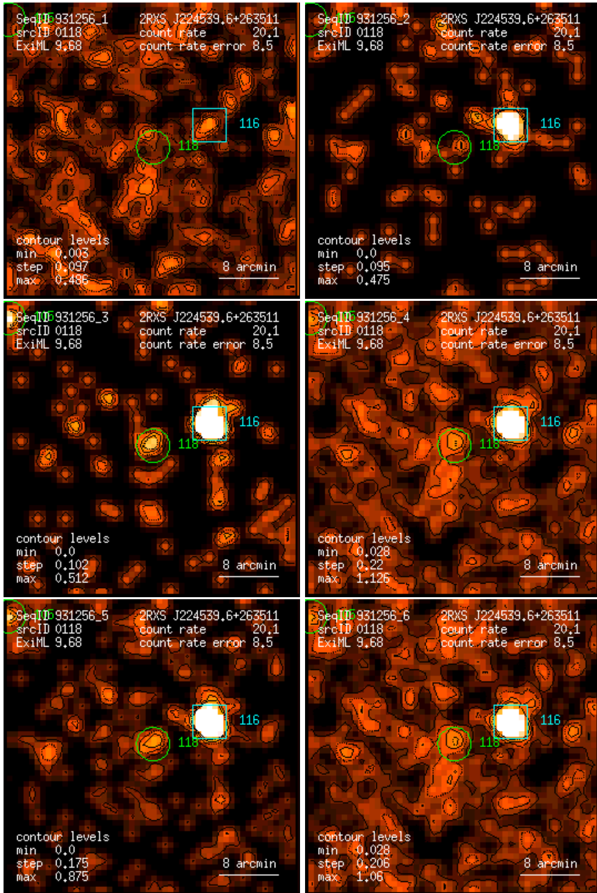
Figure 118: RASS 931256: detection 0118: band rate images, Gaussian filter: (1) PSPC channels 11 – 41, (2) 52 – 90, (3) 91 – 201, (4) 11 – 235, (5) 52 – 201, (6) 11 – 201. Broad band rates in counts/ks. Band rate contour levels in counts/ks/arcmin 2 .
