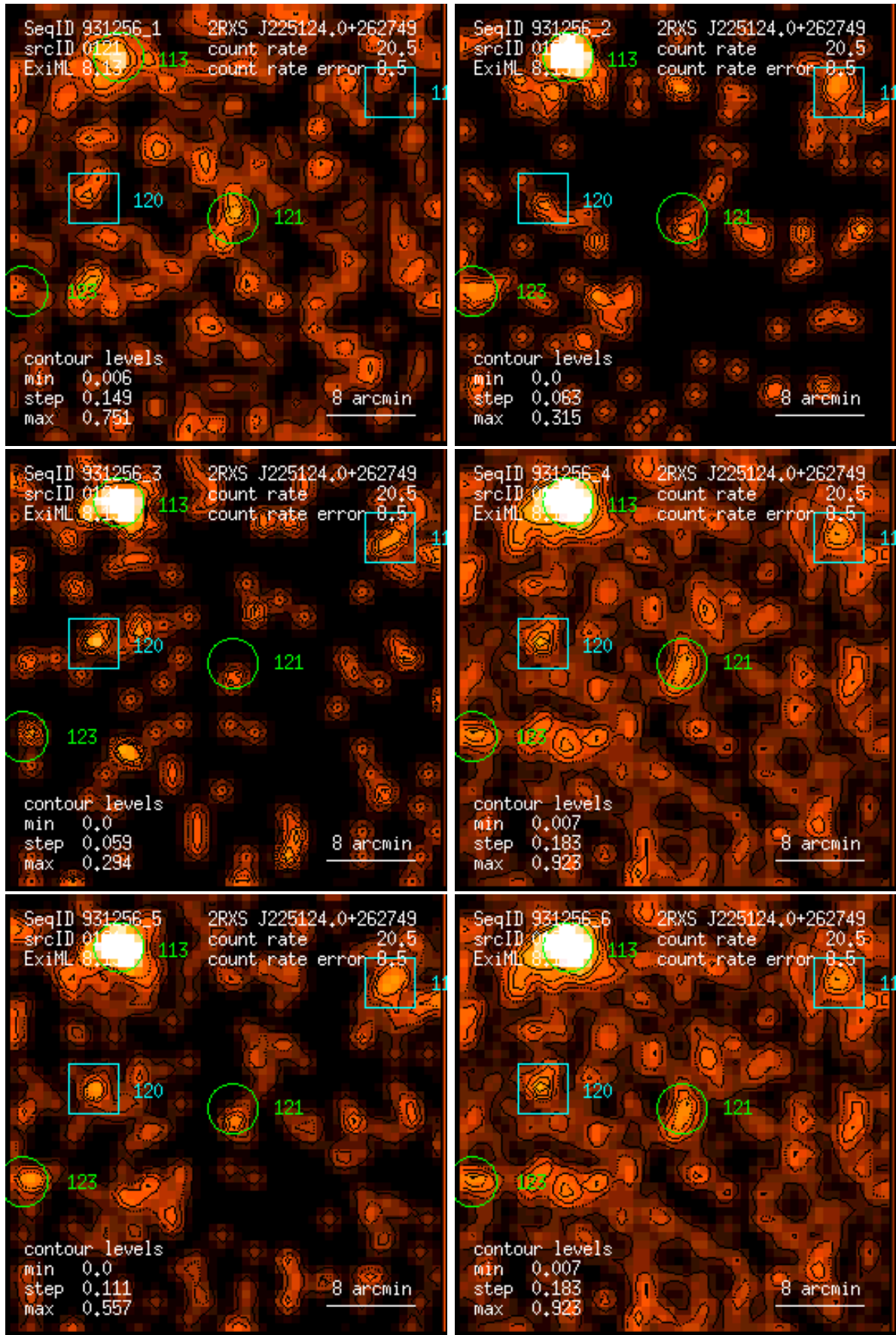
Figure 121: RASS 931256: detection 0121: band rate images, Gaussian filter: (1) PSPC channels 11 – 41, (2) 52 – 90, (3) 91 – 201, (4) 11 – 235, (5) 52 – 201, (6) 11 – 201. Broad band rates in counts/ks. Band rate contour levels in counts/ks/arcmin 2 .
