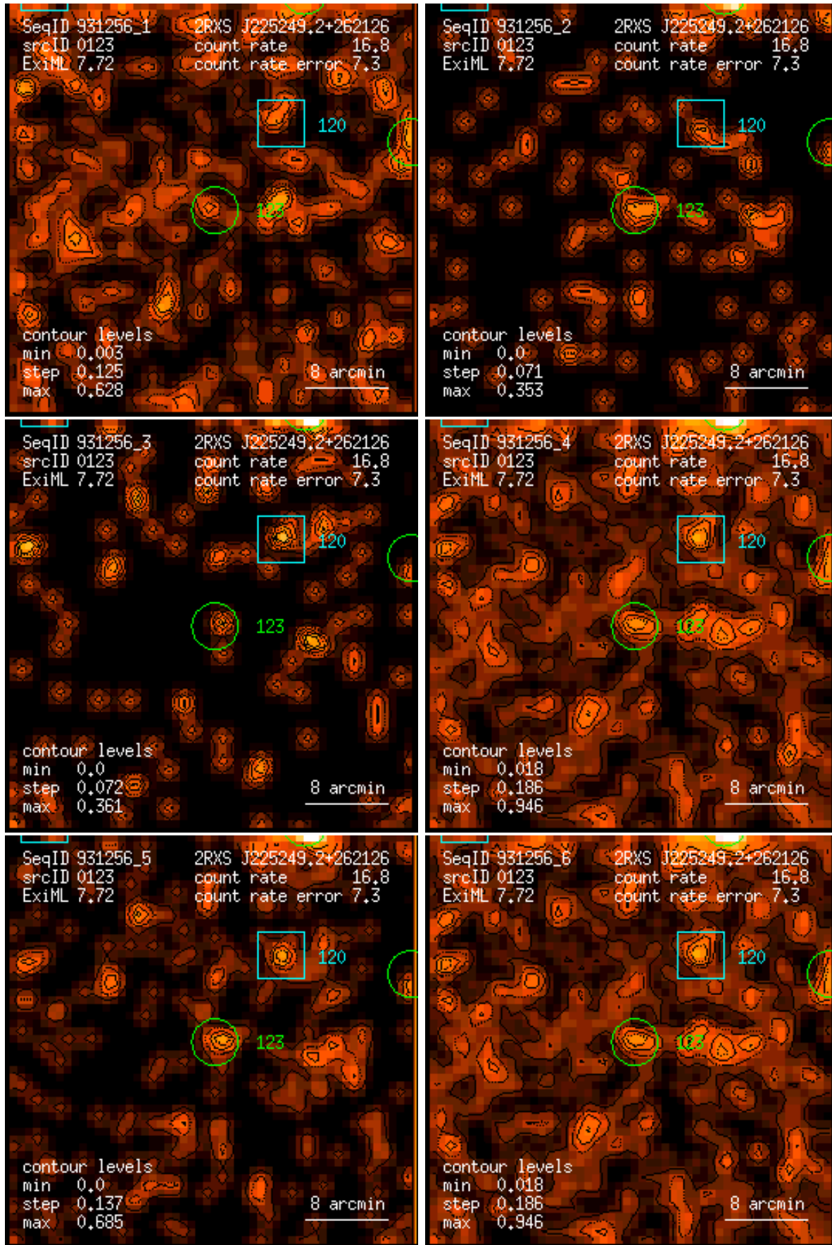
Figure 123: RASS 931256: detection 0123: band rate images, Gaussian filter: (1) PSPC channels 11 – 41, (2) 52 – 90, (3) 91 – 201, (4) 11 – 235, (5) 52 – 201, (6) 11 – 201. Broad band rates in counts/ks. Band rate contour levels in counts/ks/arcmin 2 .
