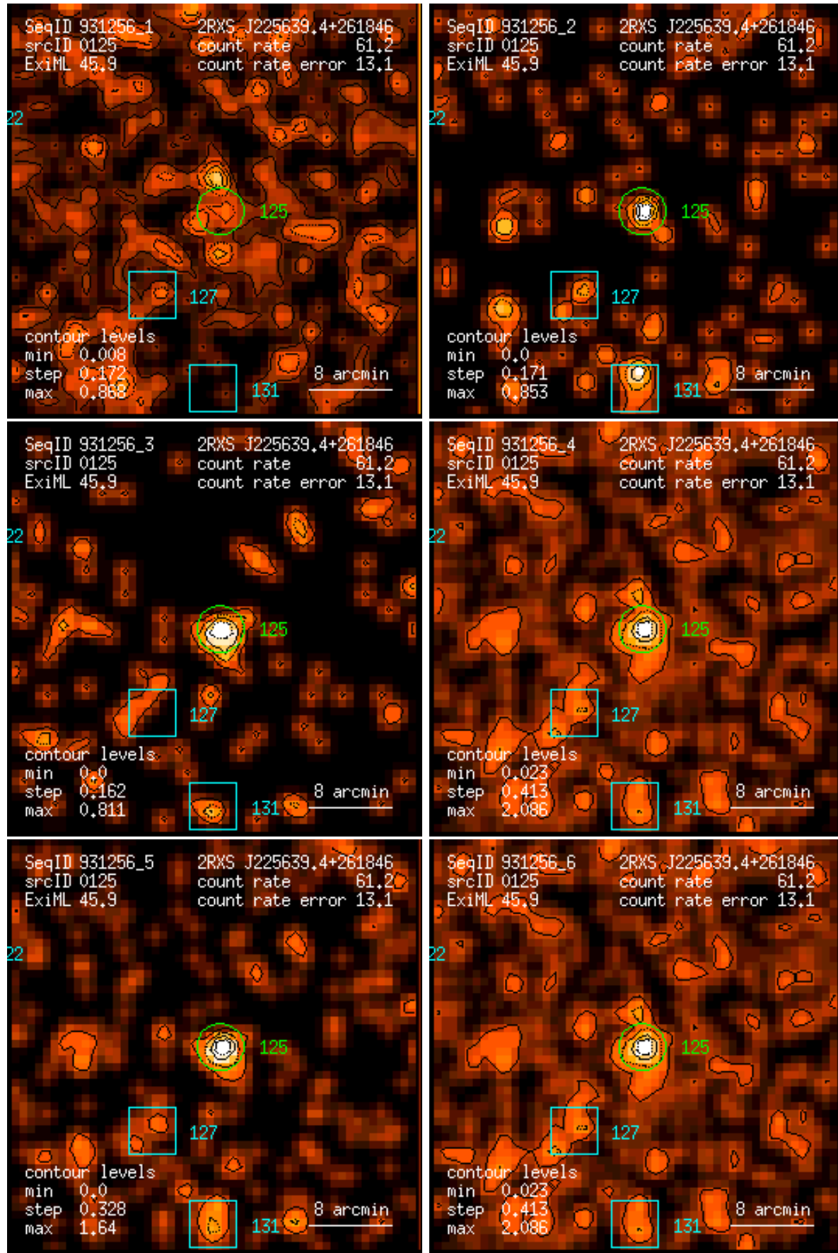
Figure 125: RASS 931256: detection 0125: band rate images, Gaussian filter: (1) PSPC channels 11 – 41, (2) 52 – 90, (3) 91 – 201, (4) 11 – 235, (5) 52 – 201, (6) 11 – 201. Broad band rates in counts/ks. Band rate contour levels in counts/ks/arcmin 2 .
