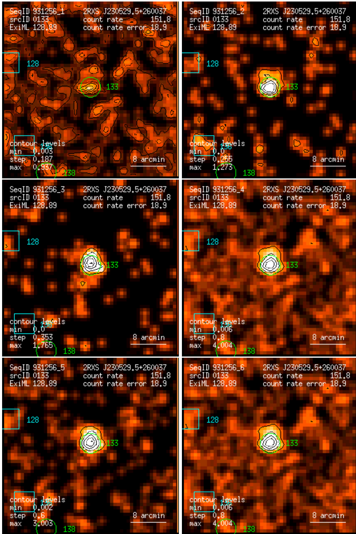
Figure 133: RASS 931256: detection 0133: band rate images, Gaussian filter: (1) PSPC channels 11 – 41, (2) 52 – 90, (3) 91 – 201, (4) 11 – 235, (5) 52 – 201, (6) 11 – 201. Broad band rates in counts/ks. Band rate contour levels in counts/ks/arcmin 2 .
