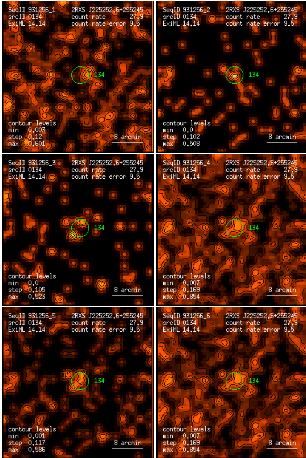
Figure 134: RASS 931256: detection 0134: band rate images, Gaussian filter: (1) PSPC channels 11 – 41, (2) 52 – 90, (3) 91 – 201, (4) 11 – 235, (5) 52 – 201, (6) 11 – 201. Broad band rates in counts/ks. Band rate contour levels in counts/ks/arcmin 2 .
