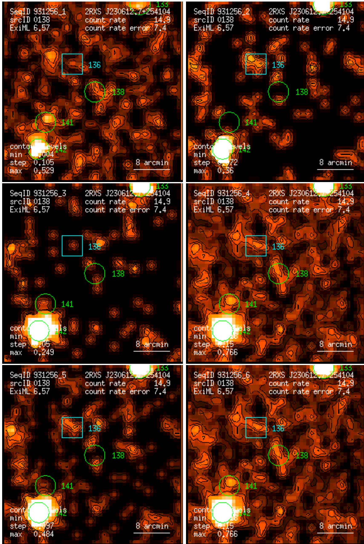
Figure 138: RASS 931256: detection 0138: band rate images, Gaussian filter: (1) PSPC channels 11 – 41, (2) 52 – 90, (3) 91 – 201, (4) 11 – 235, (5) 52 – 201, (6) 11 – 201. Broad band rates in counts/ks. Band rate contour levels in counts/ks/arcmin 2 .
