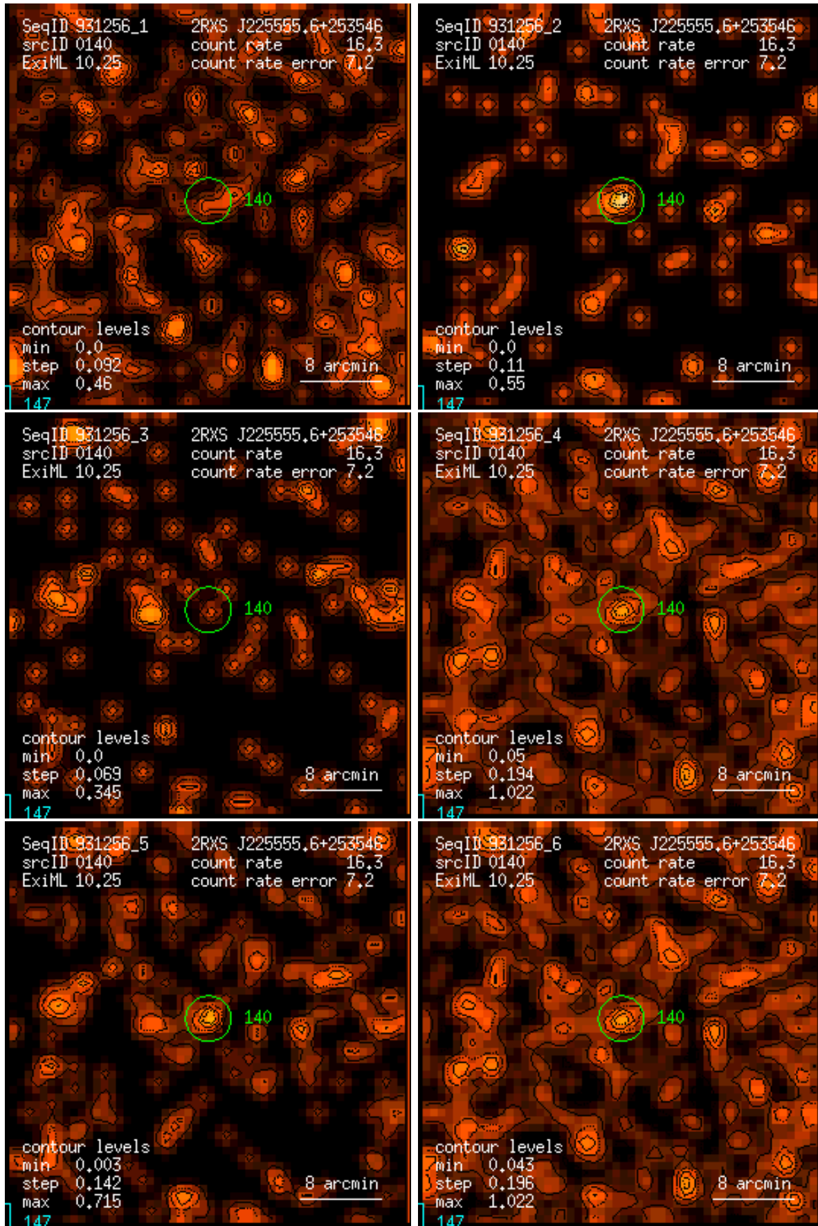
Figure 140: RASS 931256: detection 0140: band rate images, Gaussian filter: (1) PSPC channels 11 – 41, (2) 52 – 90, (3) 91 – 201, (4) 11 – 235, (5) 52 – 201, (6) 11 – 201. Broad band rates in counts/ks. Band rate contour levels in counts/ks/arcmin 2 .
