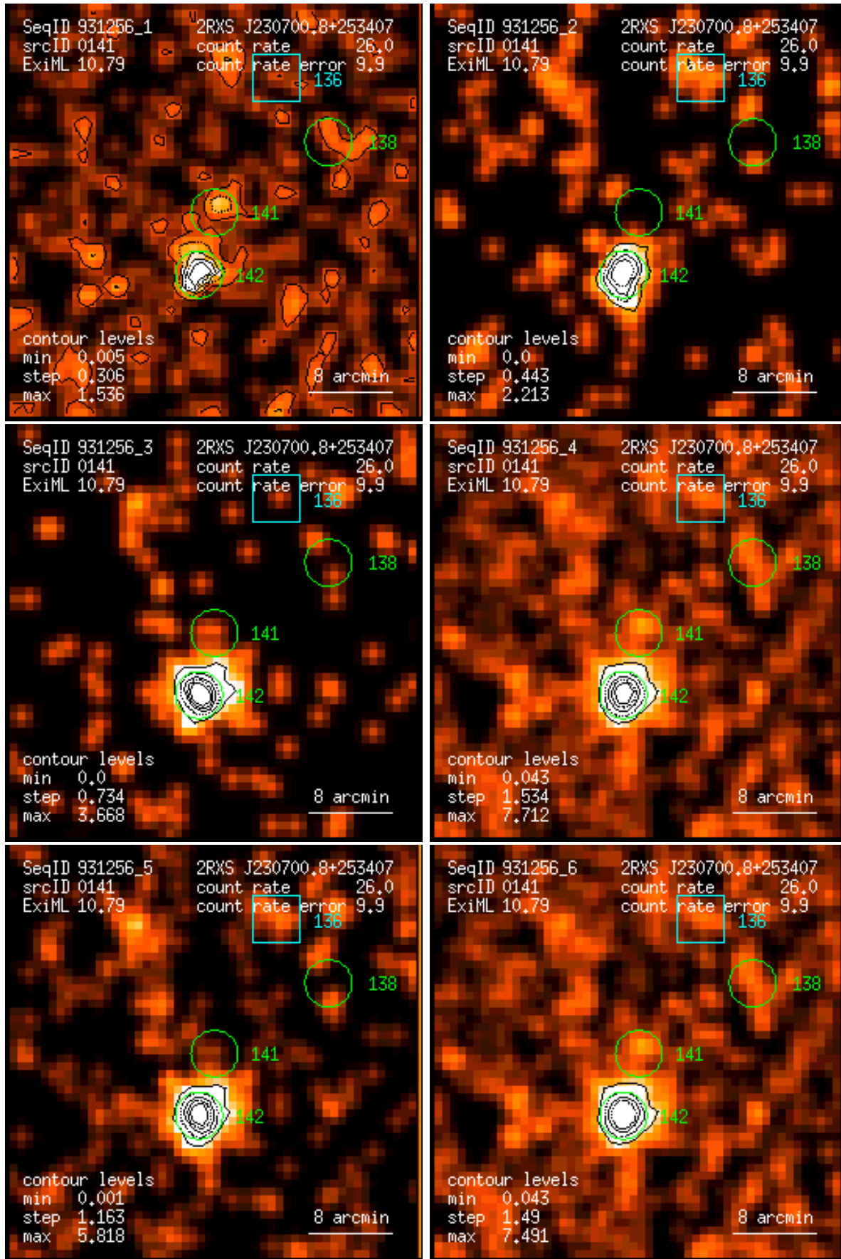
Figure 141: RASS 931256: detection 0141: band rate images, Gaussian filter: (1) PSPC channels 11 – 41, (2) 52 – 90, (3) 91 – 201, (4) 11 – 235, (5) 52 – 201, (6) 11 – 201. Broad band rates in counts/ks. Band rate contour levels in counts/ks/arcmin 2 .
