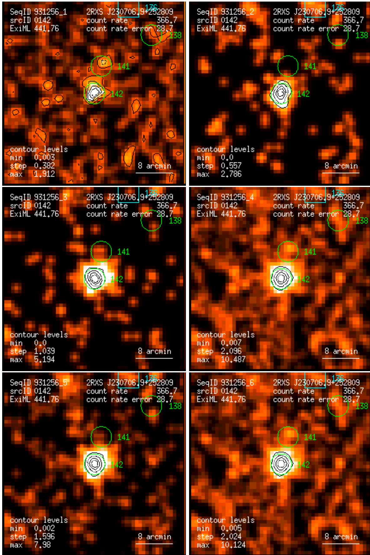
Figure 142: RASS 931256: detection 0142: band rate images, Gaussian filter: (1) PSPC channels 11 – 41, (2) 52 – 90, (3) 91 – 201, (4) 11 – 235, (5) 52 – 201, (6) 11 – 201. Broad band rates in counts/ks. Band rate contour levels in counts/ks/arcmin 2 .
