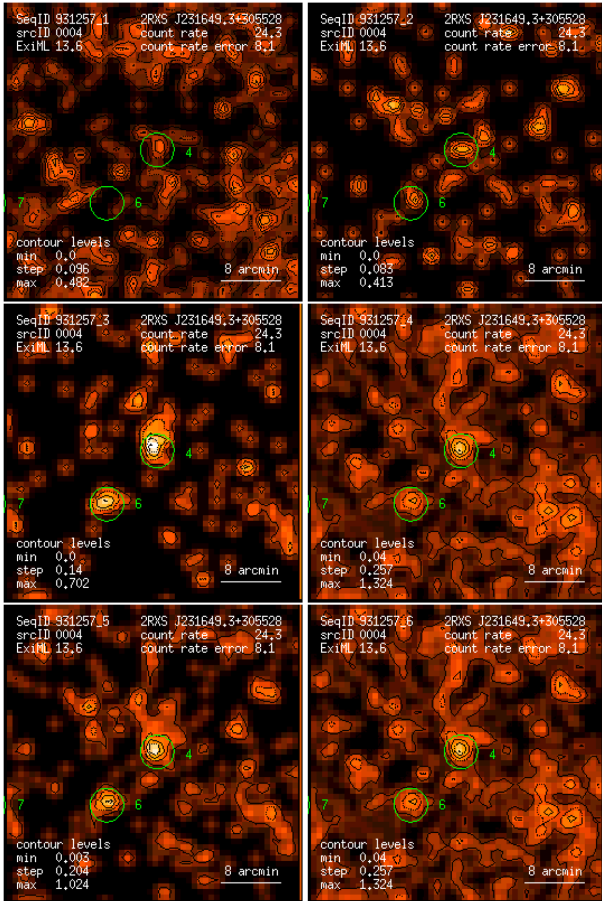
Figure 4: RASS 931257: detection 0004: band rate images, Gaussian filter: (1) PSPC channels 11 – 41, (2) 52 – 90, (3) 91 – 201, (4) 11 – 235, (5) 52 – 201, (6) 11 – 201. Broad band rates in counts/ks. Band rate contour levels in counts/ks/arcmin 2 .
