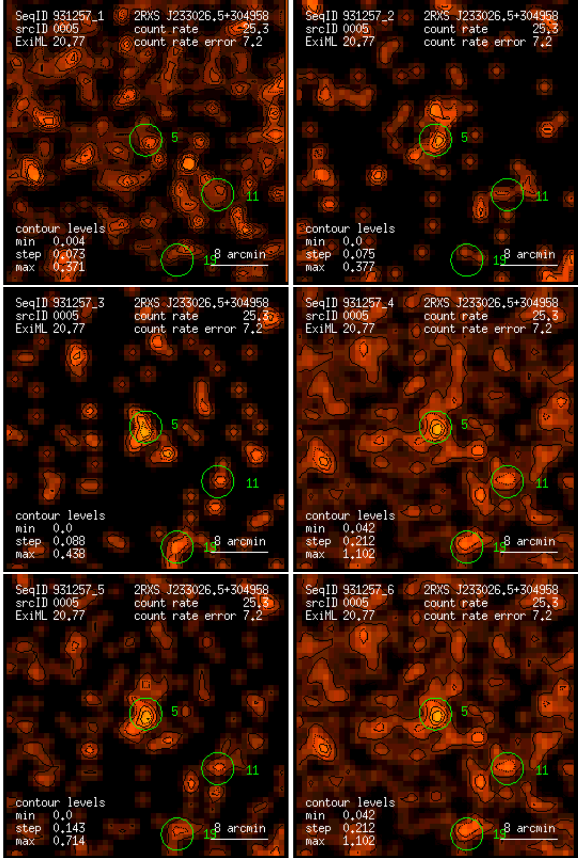
Figure 5: RASS 931257: detection 0005: band rate images, Gaussian filter: (1) PSPC channels 11 – 41, (2) 52 – 90, (3) 91 – 201, (4) 11 – 235, (5) 52 – 201, (6) 11 – 201. Broad band rates in counts/ks. Band rate contour levels in counts/ks/arcmin 2 .
