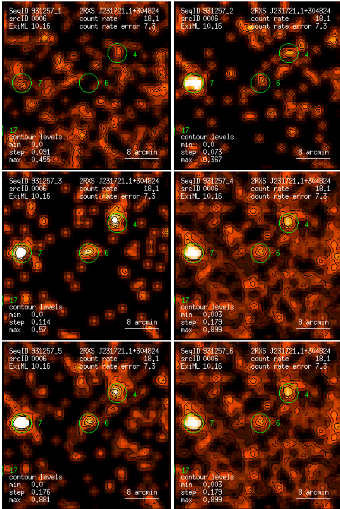
Figure 6: RASS 931257: detection 0006: band rate images, Gaussian filter: (1) PSPC channels 11 – 41, (2) 52 – 90, (3) 91 – 201, (4) 11 – 235, (5) 52 – 201, (6) 11 – 201. Broad band rates in counts/ks. Band rate contour levels in counts/ks/arcmin 2 .
