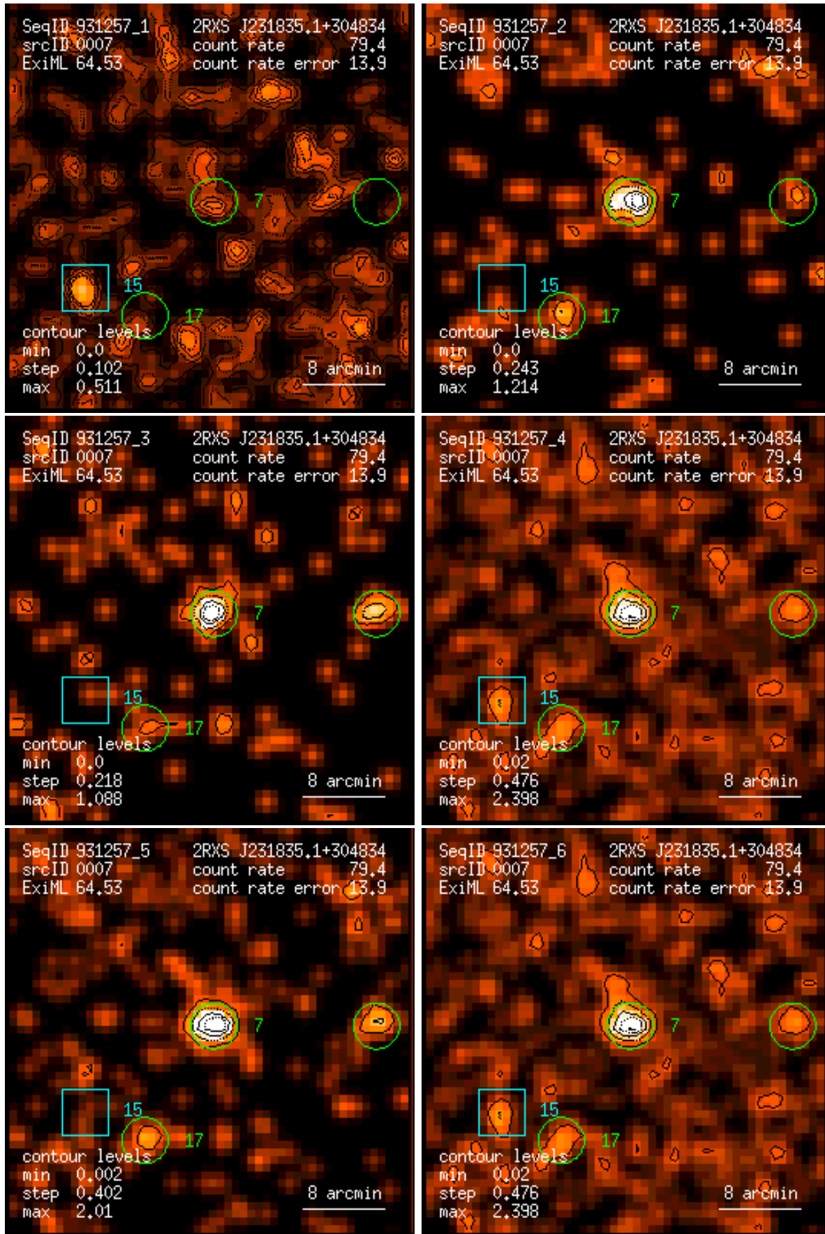
Figure 7: RASS 931257: detection 0007: band rate images, Gaussian filter: (1) PSPC channels 11 – 41, (2) 52 – 90, (3) 91 – 201, (4) 11 – 235, (5) 52 – 201, (6) 11 – 201. Broad band rates in counts/ks. Band rate contour levels in counts/ks/arcmin 2 .
