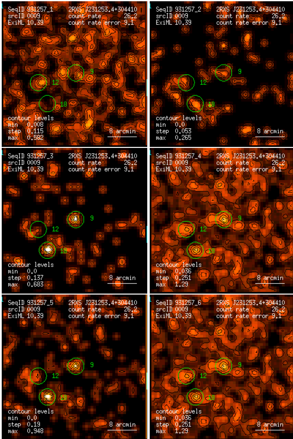
Figure 9: RASS 931257: detection 0009: band rate images, Gaussian filter: (1) PSPC channels 11 – 41, (2) 52 – 90, (3) 91 – 201, (4) 11 – 235, (5) 52 – 201, (6) 11 – 201. Broad band rates in counts/ks. Band rate contour levels in counts/ks/arcmin 2 .
