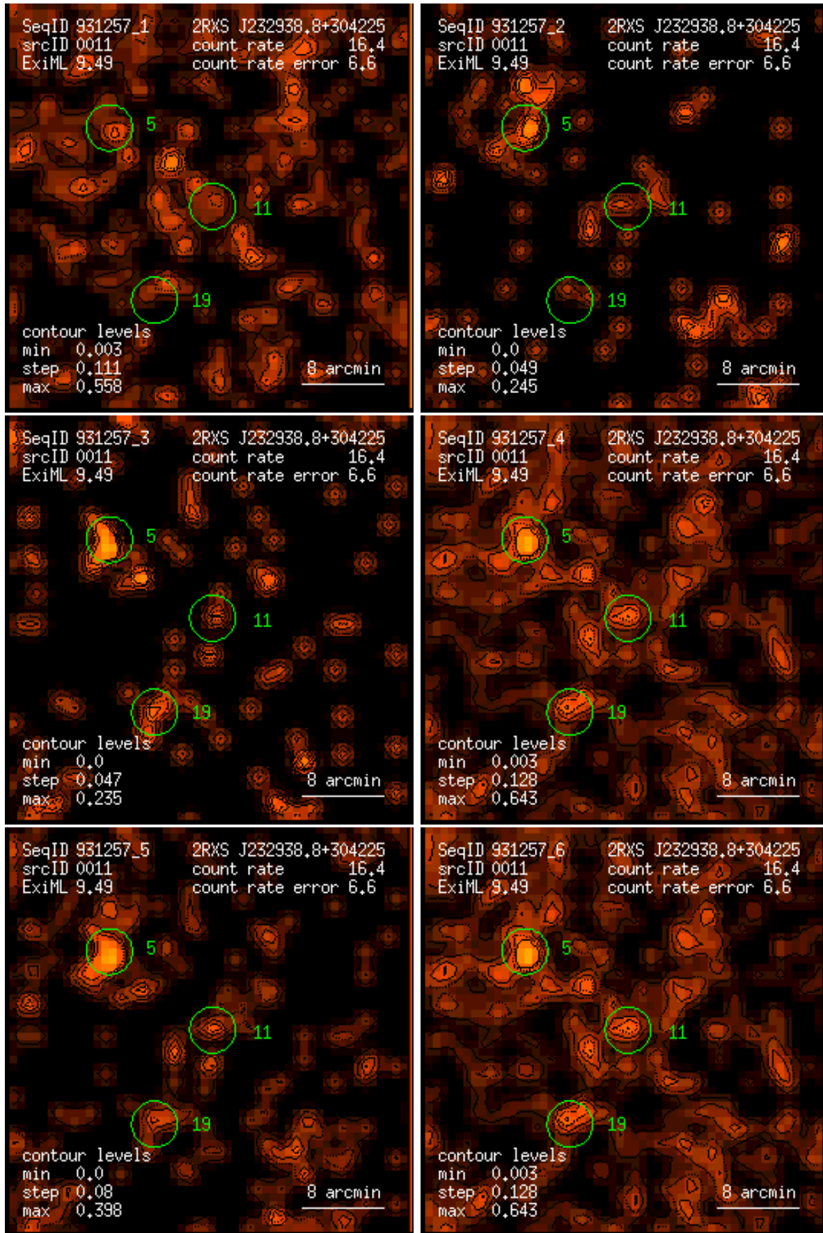
Figure 11: RASS 931257: detection 0011: band rate images, Gaussian filter: (1) PSPC channels 11 – 41, (2) 52 – 90, (3) 91 – 201, (4) 11 – 235, (5) 52 – 201, (6) 11 – 201. Broad band rates in counts/ks. Band rate contour levels in counts/ks/arcmin 2 .
